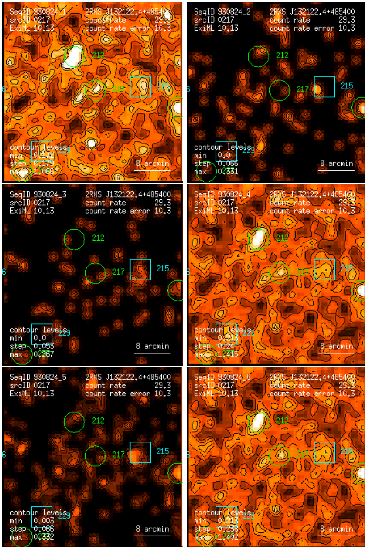
Figure 217: RASS 930824: detection 0217: band rate images, Gaussian filter: (1) PSPC channels 11 – 41, (2) 52 – 90, (3) 91 – 201, (4) 11 – 235, (5) 52 – 201, (6) 11 – 201. Broad band rates in counts/ks. Band rate contour levels in counts/ks/arcmin 2 .
