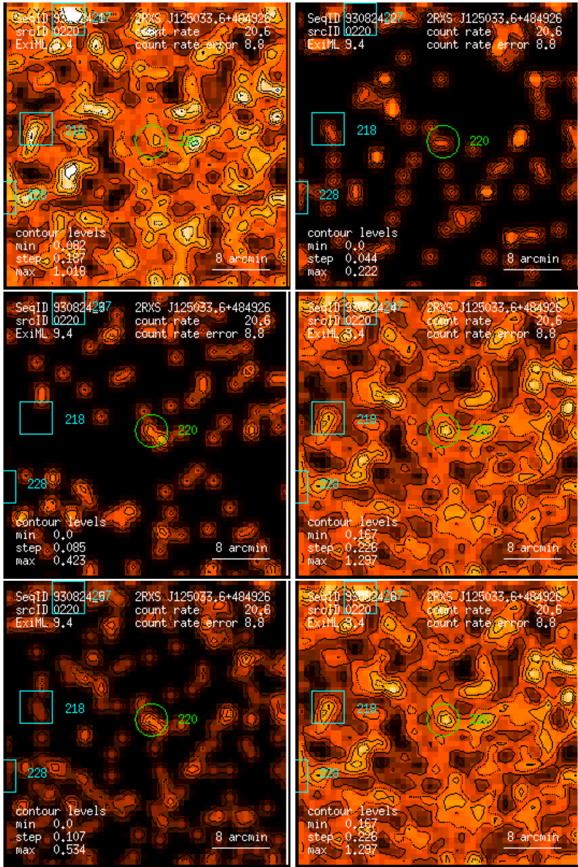
Figure 220: RASS 930824: detection 0220: band rate images, Gaussian filter: (1) PSPC channels 11 – 41, (2) 52 – 90, (3) 91 – 201, (4) 11 – 235, (5) 52 – 201, (6) 11 – 201. Broad band rates in counts/ks. Band rate contour levels in counts/ks/arcmin 2 .
