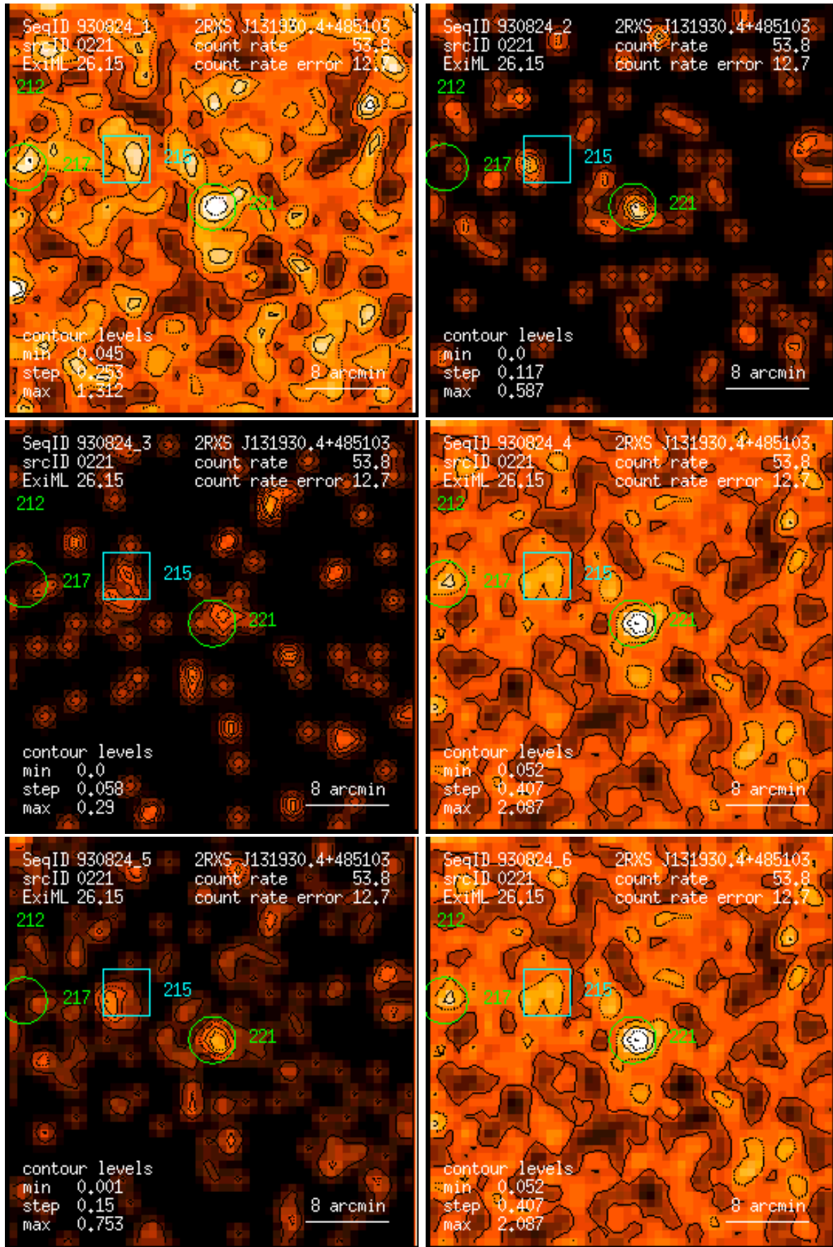
Figure 221: RASS 930824: detection 0221: band rate images, Gaussian filter: (1) PSPC channels 11 – 41, (2) 52 – 90, (3) 91 – 201, (4) 11 – 235, (5) 52 – 201, (6) 11 – 201. Broad band rates in counts/ks. Band rate contour levels in counts/ks/arcmin 2 .
