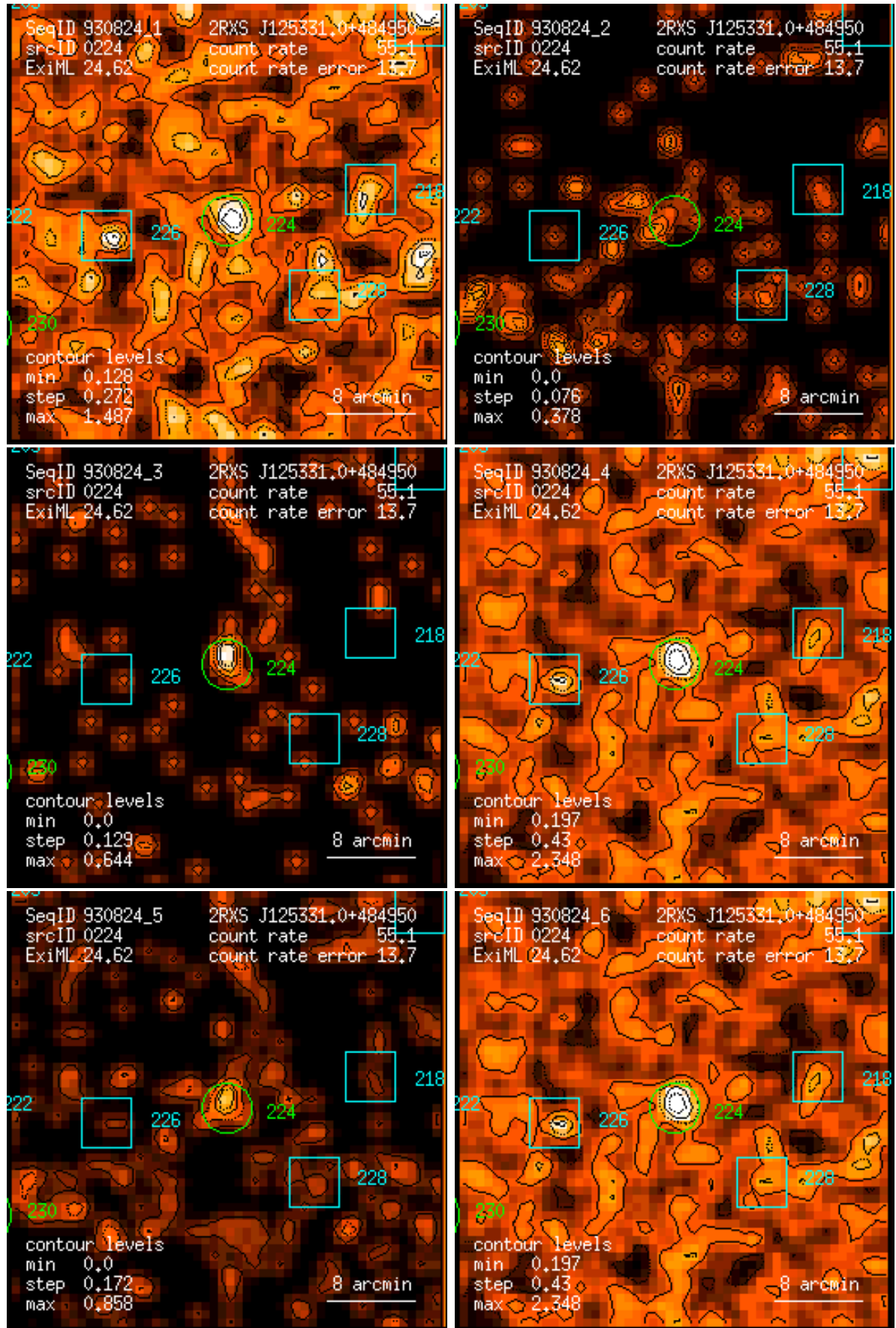
Figure 224: RASS 930824: detection 0224: band rate images, Gaussian filter: (1) PSPC channels 11 – 41, (2) 52 – 90, (3) 91 – 201, (4) 11 – 235, (5) 52 – 201, (6) 11 – 201. Broad band rates in counts/ks. Band rate contour levels in counts/ks/arcmin 2 .
