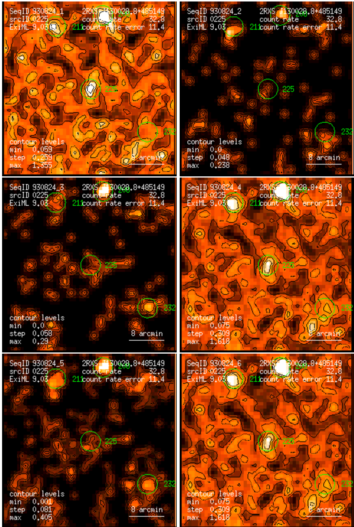
Figure 225: RASS 930824: detection 0225: band rate images, Gaussian filter: (1) PSPC channels 11 – 41, (2) 52 – 90, (3) 91 – 201, (4) 11 – 235, (5) 52 – 201, (6) 11 – 201. Broad band rates in counts/ks. Band rate contour levels in counts/ks/arcmin 2 .
