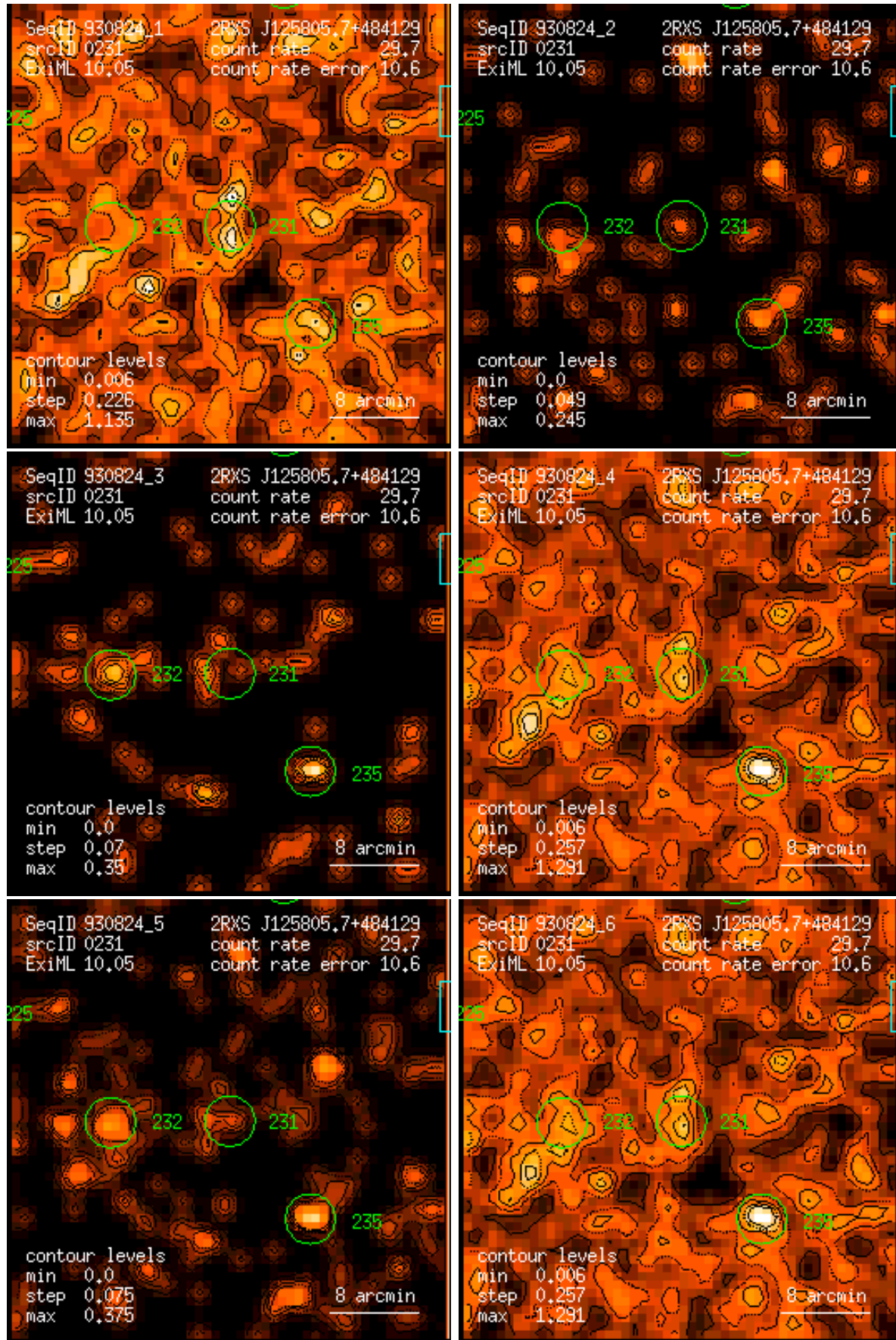
Figure 231: RASS 930824: detection 0231: band rate images, Gaussian filter: (1) PSPC channels 11 – 41, (2) 52 – 90, (3) 91 – 201, (4) 11 – 235, (5) 52 – 201, (6) 11 – 201. Broad band rates in counts/ks. Band rate contour levels in counts/ks/arcmin 2 .
