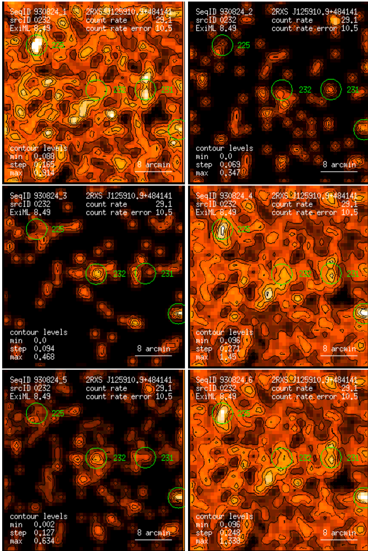
Figure 232: RASS 930824: detection 0232: band rate images, Gaussian filter: (1) PSPC channels 11 – 41, (2) 52 – 90, (3) 91 – 201, (4) 11 – 235, (5) 52 – 201, (6) 11 – 201. Broad band rates in counts/ks. Band rate contour levels in counts/ks/arcmin 2 .
