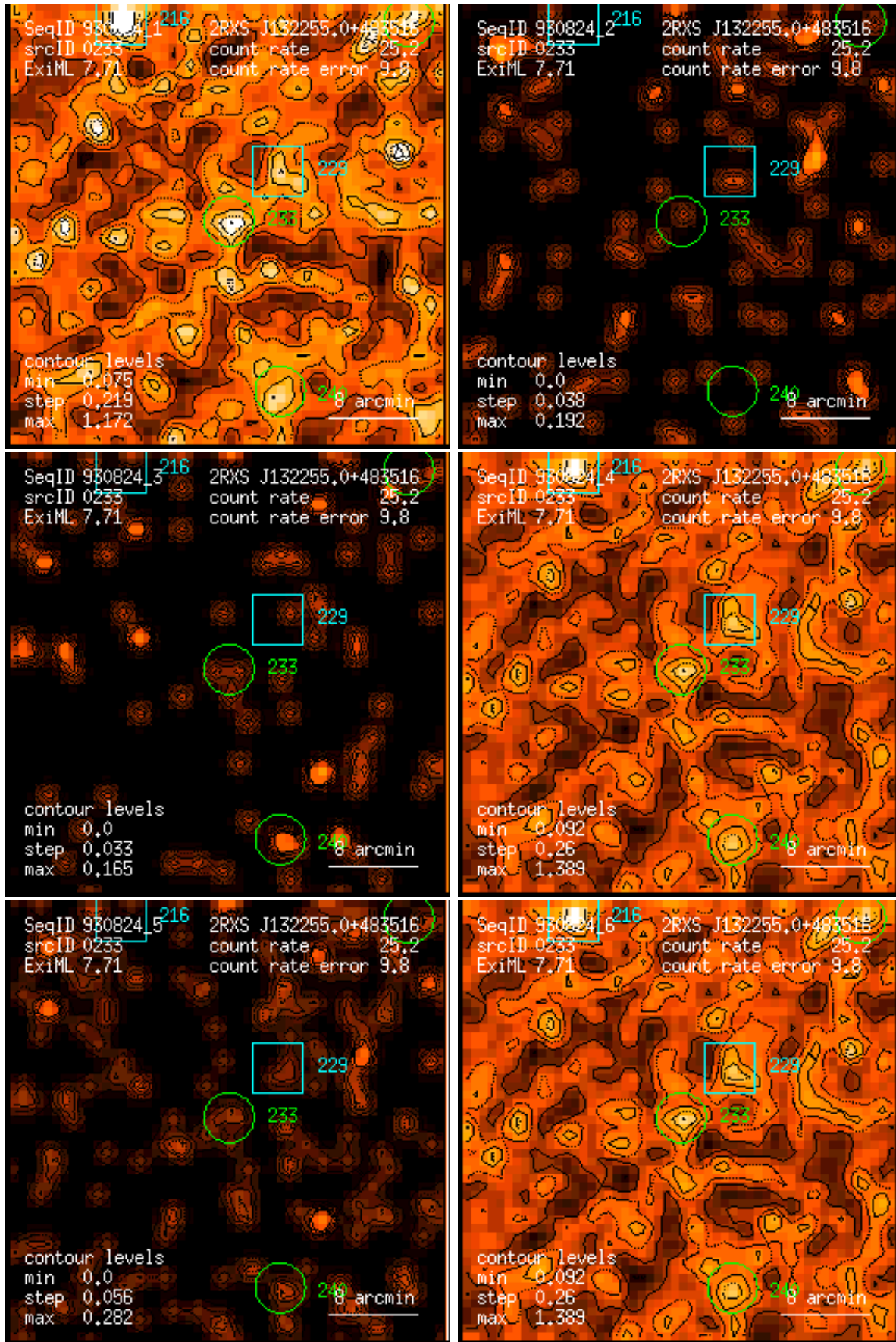
Figure 233: RASS 930824: detection 0233: band rate images, Gaussian filter: (1) PSPC channels 11 – 41, (2) 52 – 90, (3) 91 – 201, (4) 11 – 235, (5) 52 – 201, (6) 11 – 201. Broad band rates in counts/ks. Band rate contour levels in counts/ks/arcmin 2 .
