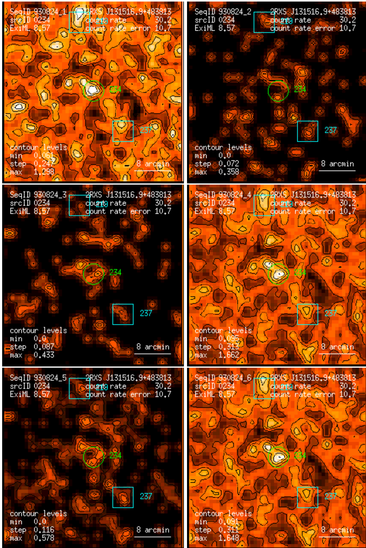
Figure 234: RASS 930824: detection 0234: band rate images, Gaussian filter: (1) PSPC channels 11 – 41, (2) 52 – 90, (3) 91 – 201, (4) 11 – 235, (5) 52 – 201, (6) 11 – 201. Broad band rates in counts/ks. Band rate contour levels in counts/ks/arcmin 2 .
