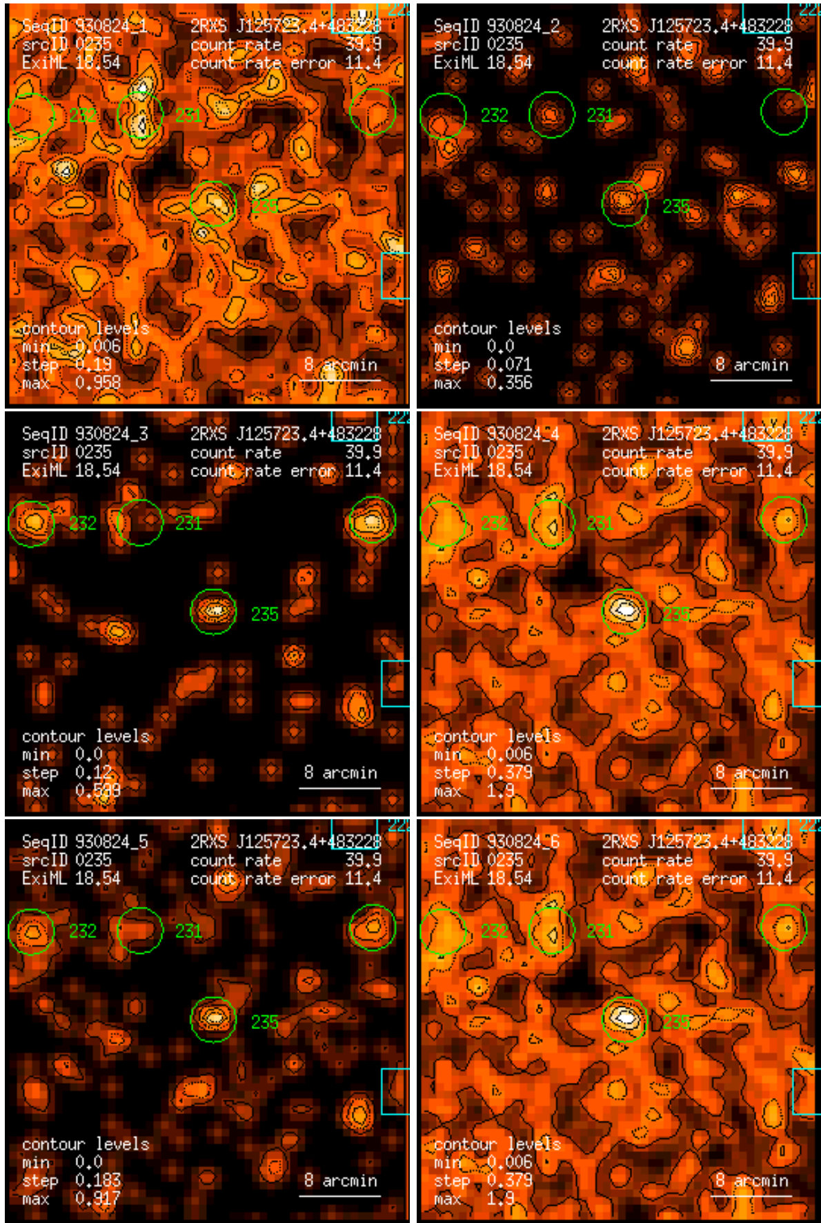
Figure 235: RASS 930824: detection 0235: band rate images, Gaussian filter: (1) PSPC channels 11 – 41, (2) 52 – 90, (3) 91 – 201, (4) 11 – 235, (5) 52 – 201, (6) 11 – 201. Broad band rates in counts/ks. Band rate contour levels in counts/ks/arcmin 2 .
