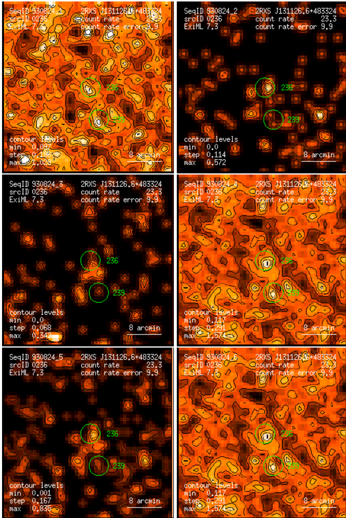
Figure 236: RASS 930824: detection 0236: band rate images, Gaussian filter: (1) PSPC channels 11 – 41, (2) 52 – 90, (3) 91 – 201, (4) 11 – 235, (5) 52 – 201, (6) 11 – 201. Broad band rates in counts/ks. Band rate contour levels in counts/ks/arcmin 2 .
