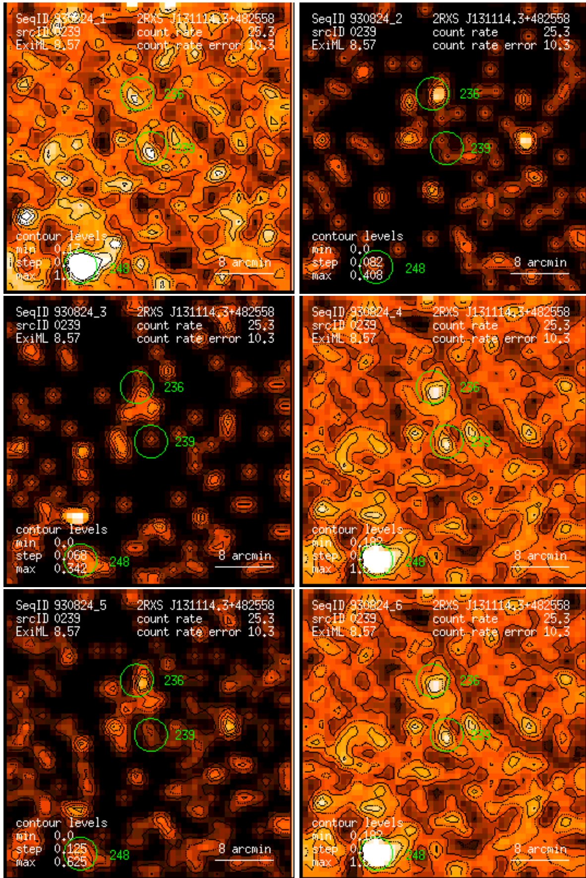
Figure 239: RASS 930824: detection 0239: band rate images, Gaussian filter: (1) PSPC channels 11 – 41, (2) 52 – 90, (3) 91 – 201, (4) 11 – 235, (5) 52 – 201, (6) 11 – 201. Broad band rates in counts/ks. Band rate contour levels in counts/ks/arcmin 2 .
