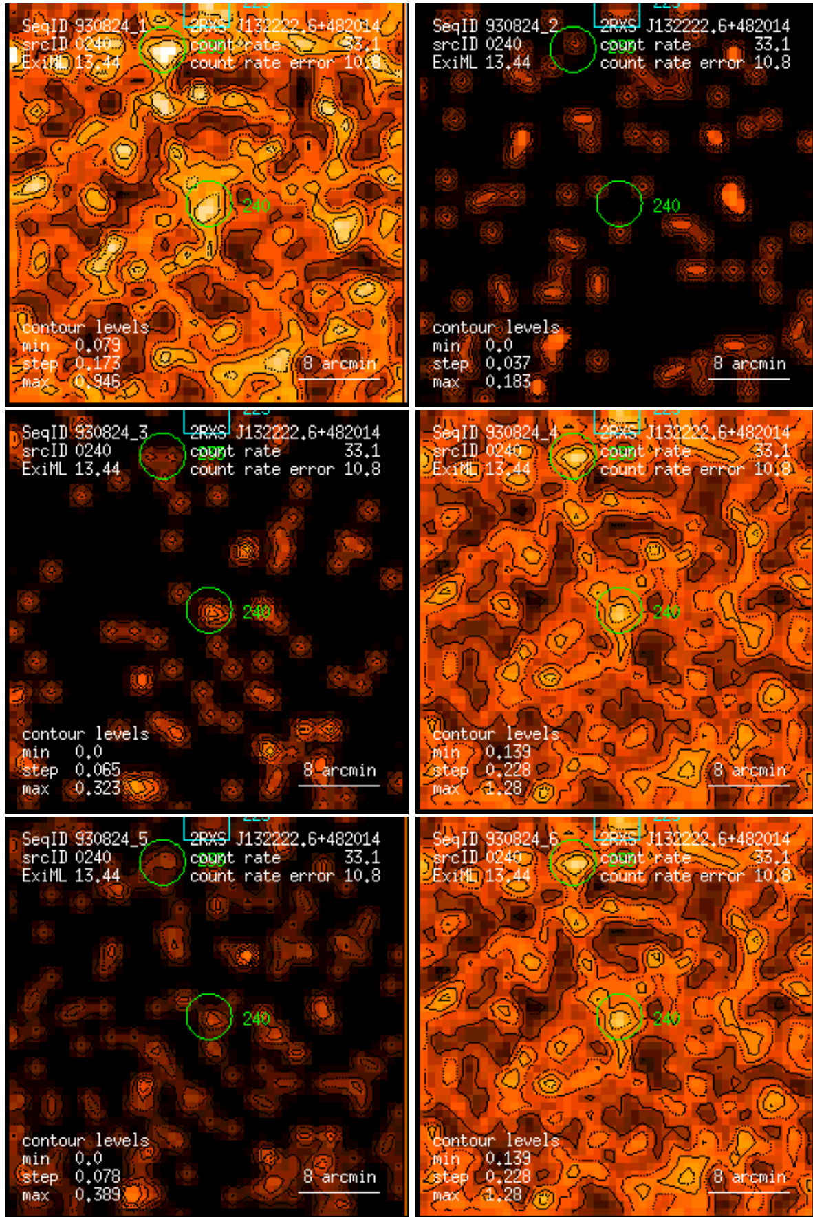
Figure 240: RASS 930824: detection 0240: band rate images, Gaussian filter: (1) PSPC channels 11 – 41, (2) 52 – 90, (3) 91 – 201, (4) 11 – 235, (5) 52 – 201, (6) 11 – 201. Broad band rates in counts/ks. Band rate contour levels in counts/ks/arcmin 2 .
