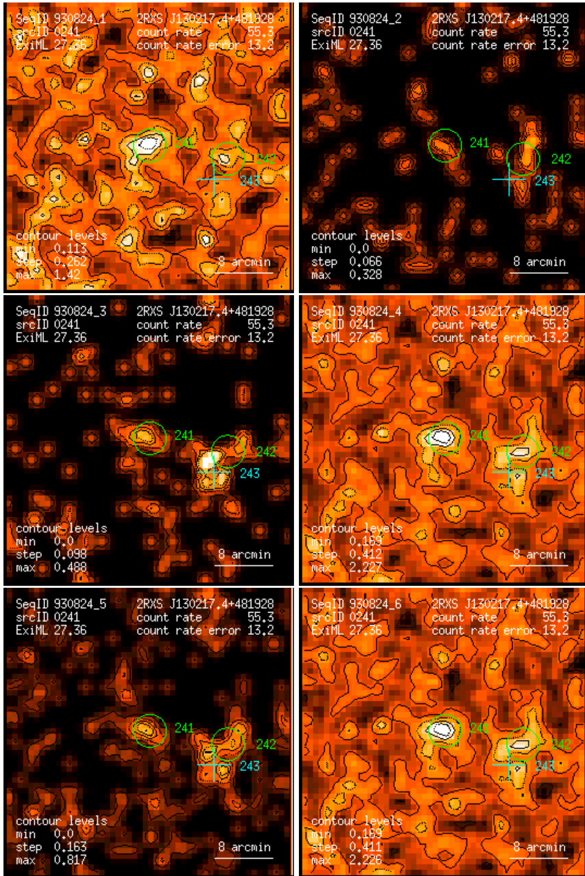
Figure 241: RASS 930824: detection 0241: band rate images, Gaussian filter: (1) PSPC channels 11 – 41, (2) 52 – 90, (3) 91 – 201, (4) 11 – 235, (5) 52 – 201, (6) 11 – 201. Broad band rates in counts/ks. Band rate contour levels in counts/ks/arcmin 2 .
