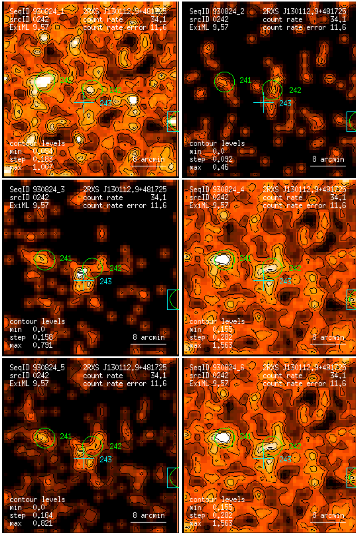
Figure 242: RASS 930824: detection 0242: band rate images, Gaussian filter: (1) PSPC channels 11 – 41, (2) 52 – 90, (3) 91 – 201, (4) 11 – 235, (5) 52 – 201, (6) 11 – 201. Broad band rates in counts/ks. Band rate contour levels in counts/ks/arcmin 2 .
