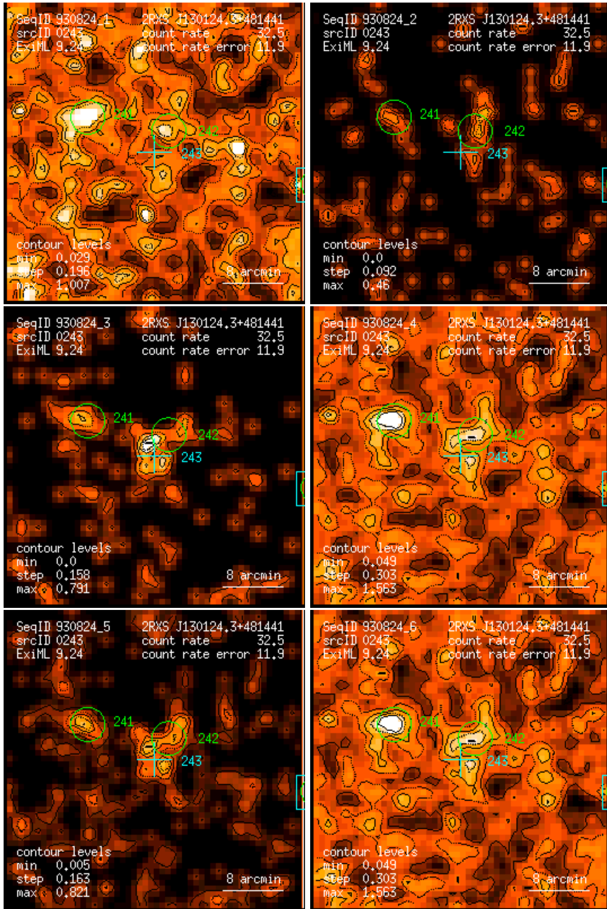
Figure 243: RASS 930824: detection 0243: band rate images, Gaussian filter: (1) PSPC channels 11 – 41, (2) 52 – 90, (3) 91 – 201, (4) 11 – 235, (5) 52 – 201, (6) 11 – 201. Broad band rates in counts/ks. Band rate contour levels in counts/ks/arcmin 2 .
