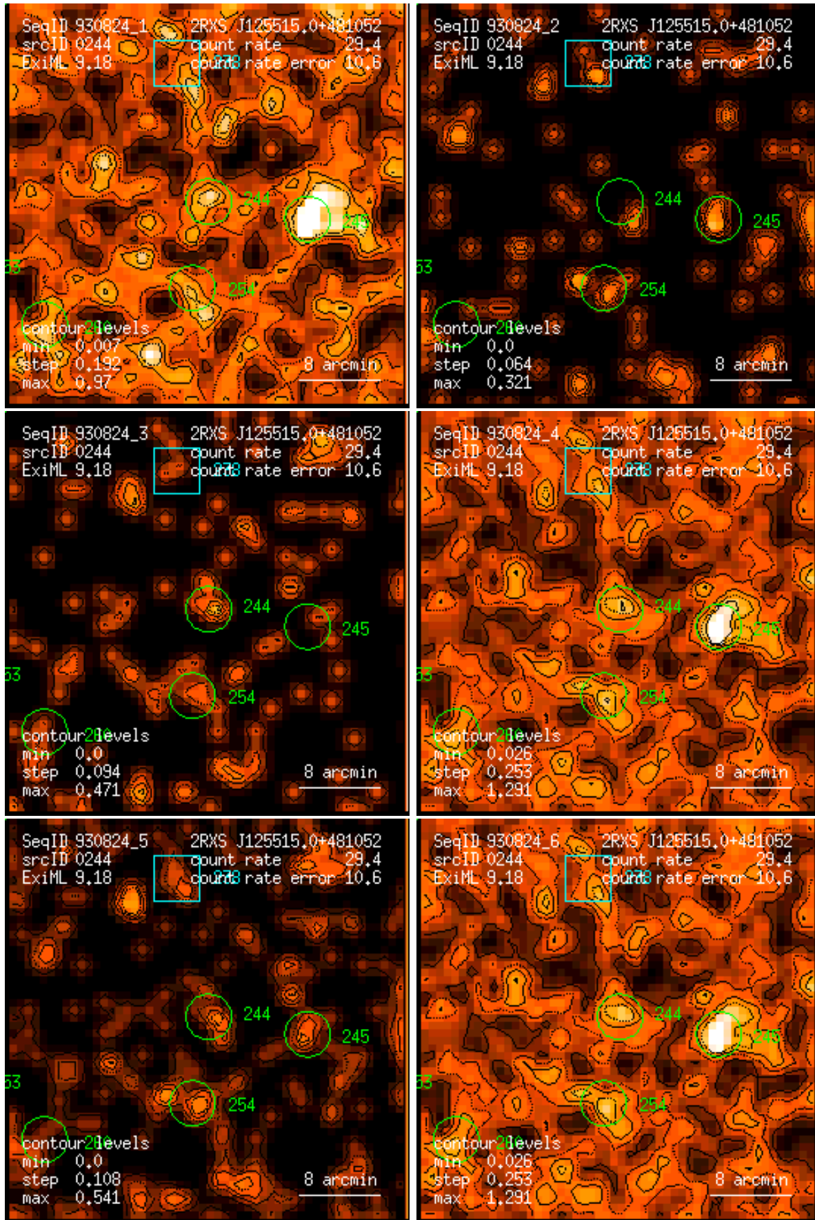
Figure 244: RASS 930824: detection 0244: band rate images, Gaussian filter: (1) PSPC channels 11 – 41, (2) 52 – 90, (3) 91 – 201, (4) 11 – 235, (5) 52 – 201, (6) 11 – 201. Broad band rates in counts/ks. Band rate contour levels in counts/ks/arcmin 2 .
