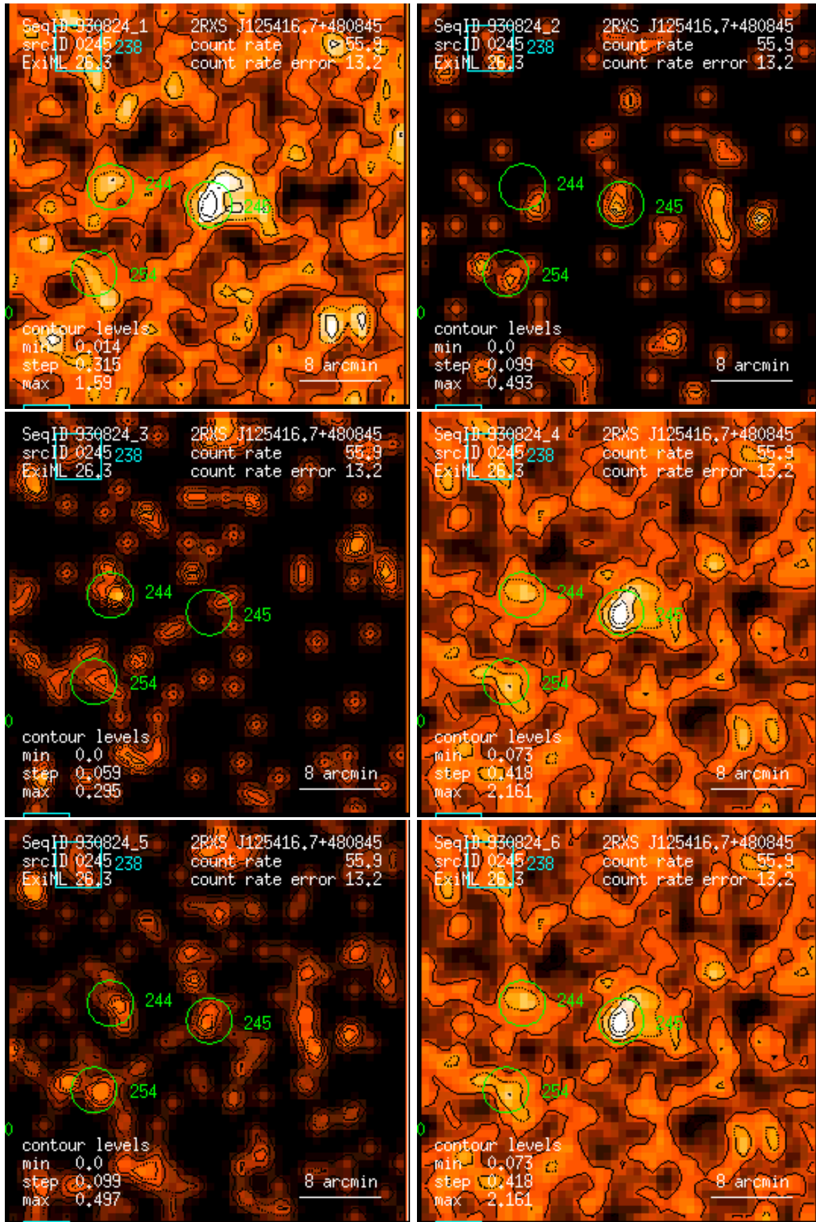
Figure 245: RASS 930824: detection 0245: band rate images, Gaussian filter: (1) PSPC channels 11 – 41, (2) 52 – 90, (3) 91 – 201, (4) 11 – 235, (5) 52 – 201, (6) 11 – 201. Broad band rates in counts/ks. Band rate contour levels in counts/ks/arcmin 2 .
