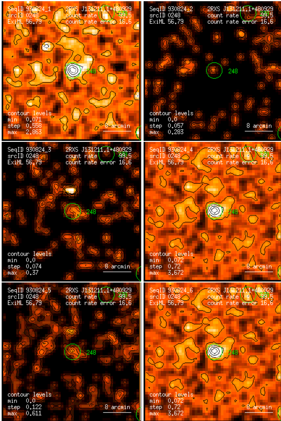
Figure 248: RASS 930824: detection 0248: band rate images, Gaussian filter: (1) PSPC channels 11 – 41, (2) 52 – 90, (3) 91 – 201, (4) 11 – 235, (5) 52 – 201, (6) 11 – 201. Broad band rates in counts/ks. Band rate contour levels in counts/ks/arcmin 2 .
