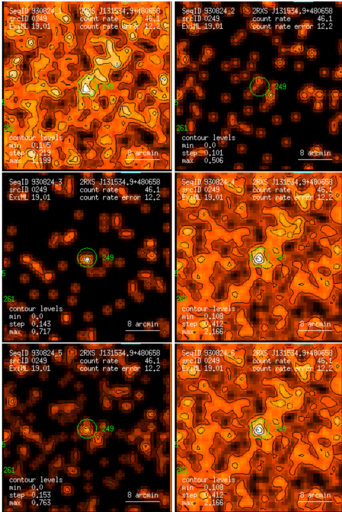
Figure 249: RASS 930824: detection 0249: band rate images, Gaussian filter: (1) PSPC channels 11 – 41, (2) 52 – 90, (3) 91 – 201, (4) 11 – 235, (5) 52 – 201, (6) 11 – 201. Broad band rates in counts/ks. Band rate contour levels in counts/ks/arcmin 2 .
