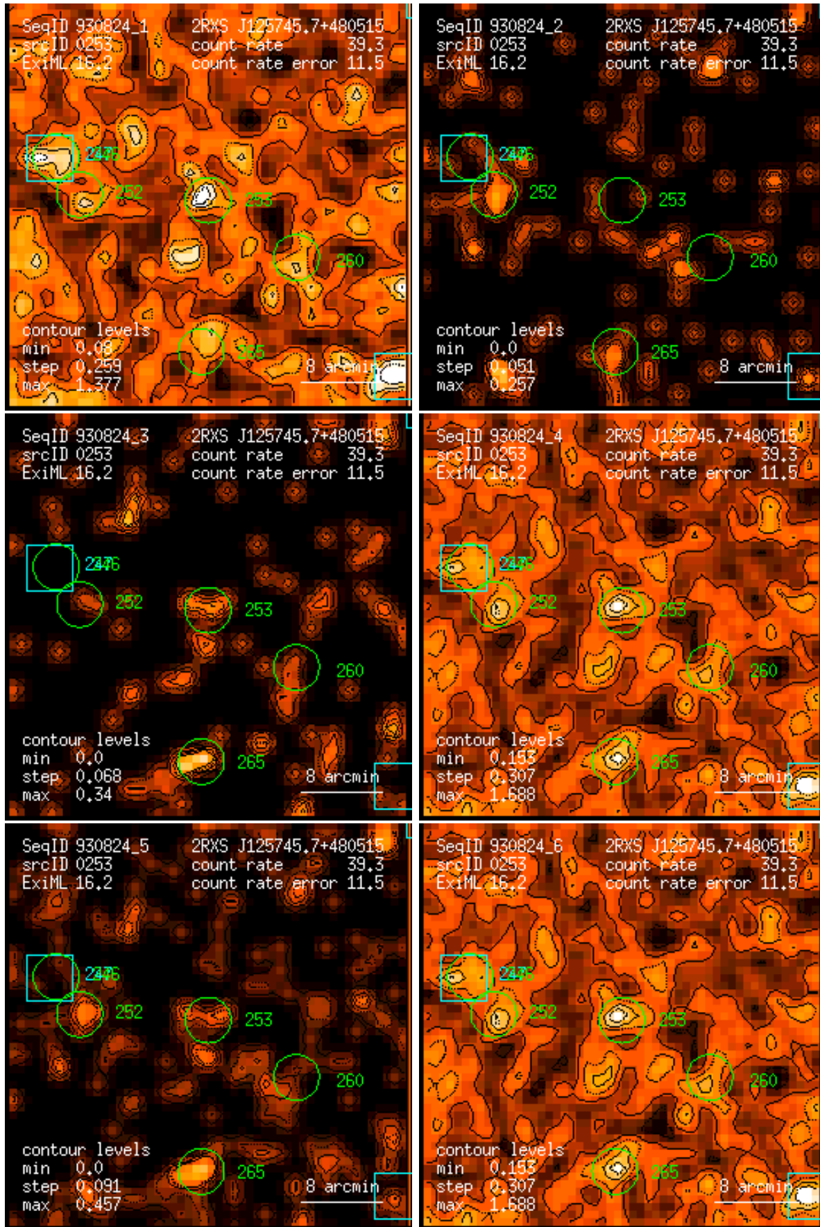
Figure 253: RASS 930824: detection 0253: band rate images, Gaussian filter: (1) PSPC channels 11 – 41, (2) 52 – 90, (3) 91 – 201, (4) 11 – 235, (5) 52 – 201, (6) 11 – 201. Broad band rates in counts/ks. Band rate contour levels in counts/ks/arcmin 2 .
