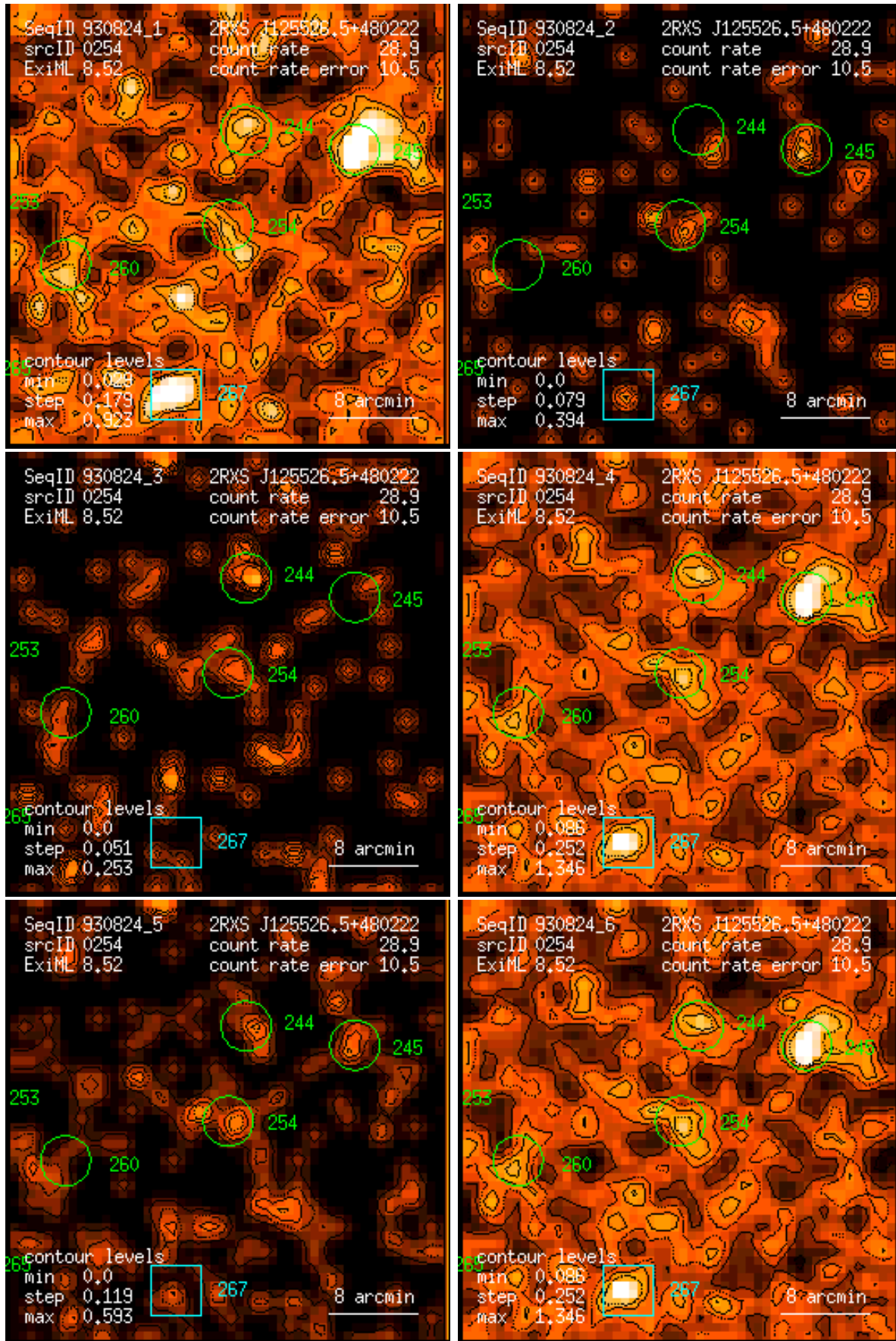
Figure 254: RASS 930824: detection 0254: band rate images, Gaussian filter: (1) PSPC channels 11 – 41, (2) 52 – 90, (3) 91 – 201, (4) 11 – 235, (5) 52 – 201, (6) 11 – 201. Broad band rates in counts/ks. Band rate contour levels in counts/ks/arcmin 2 .
