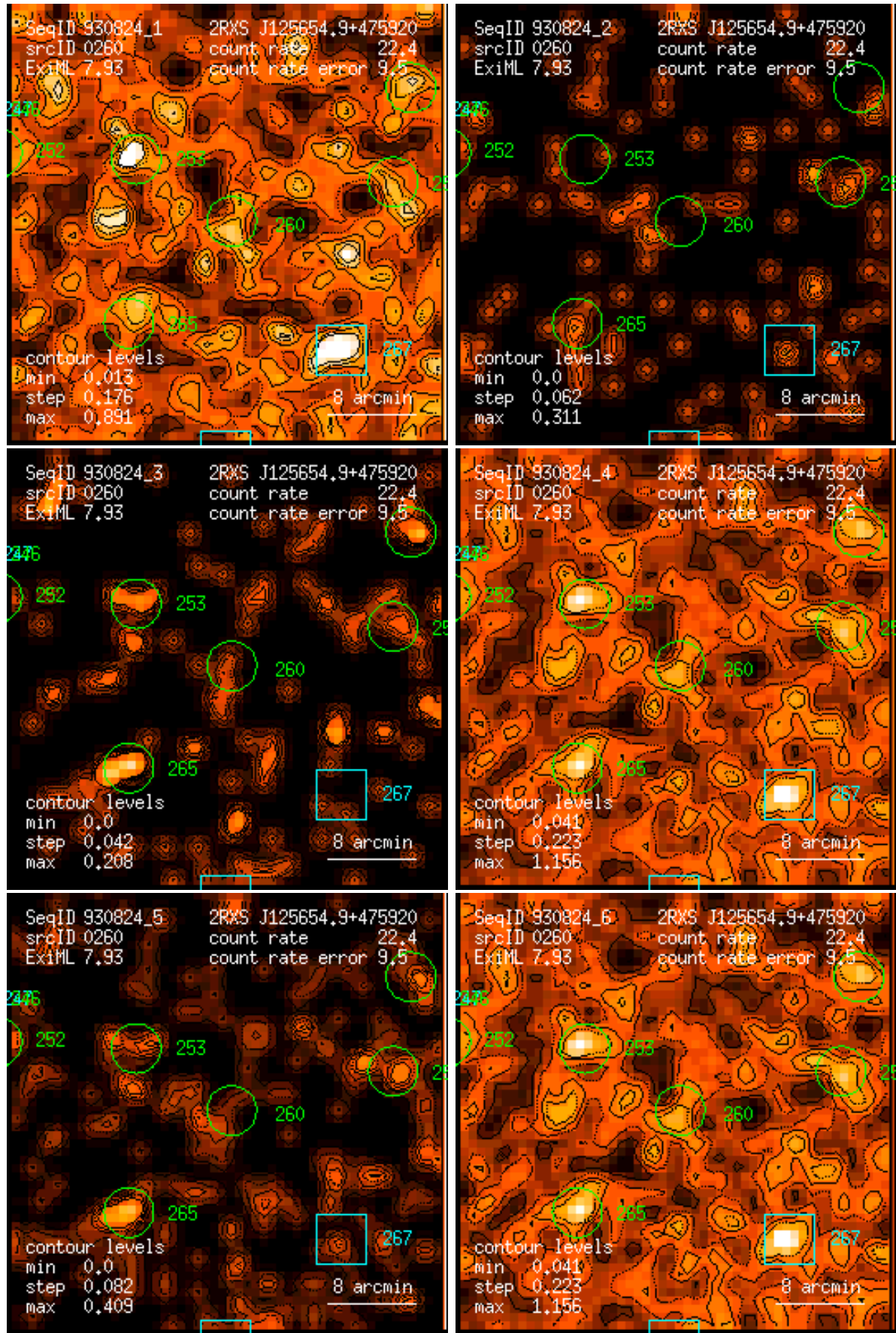
Figure 260: RASS 930824: detection 0260: band rate images, Gaussian filter: (1) PSPC channels 11 – 41, (2) 52 – 90, (3) 91 – 201, (4) 11 – 235, (5) 52 – 201, (6) 11 – 201. Broad band rates in counts/ks. Band rate contour levels in counts/ks/arcmin 2 .
