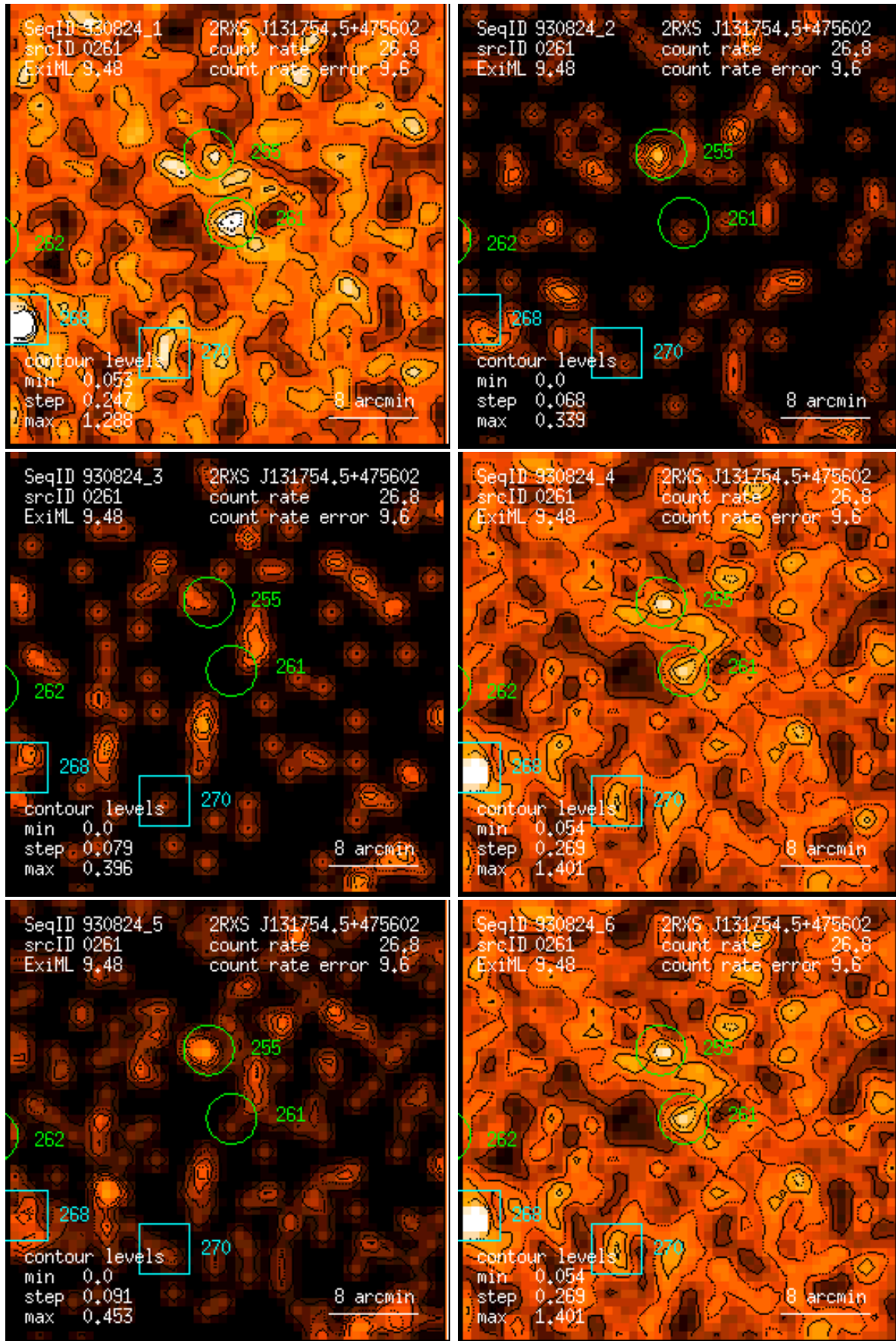
Figure 261: RASS 930824: detection 0261: band rate images, Gaussian filter: (1) PSPC channels 11 – 41, (2) 52 – 90, (3) 91 – 201, (4) 11 – 235, (5) 52 – 201, (6) 11 – 201. Broad band rates in counts/ks. Band rate contour levels in counts/ks/arcmin 2 .
