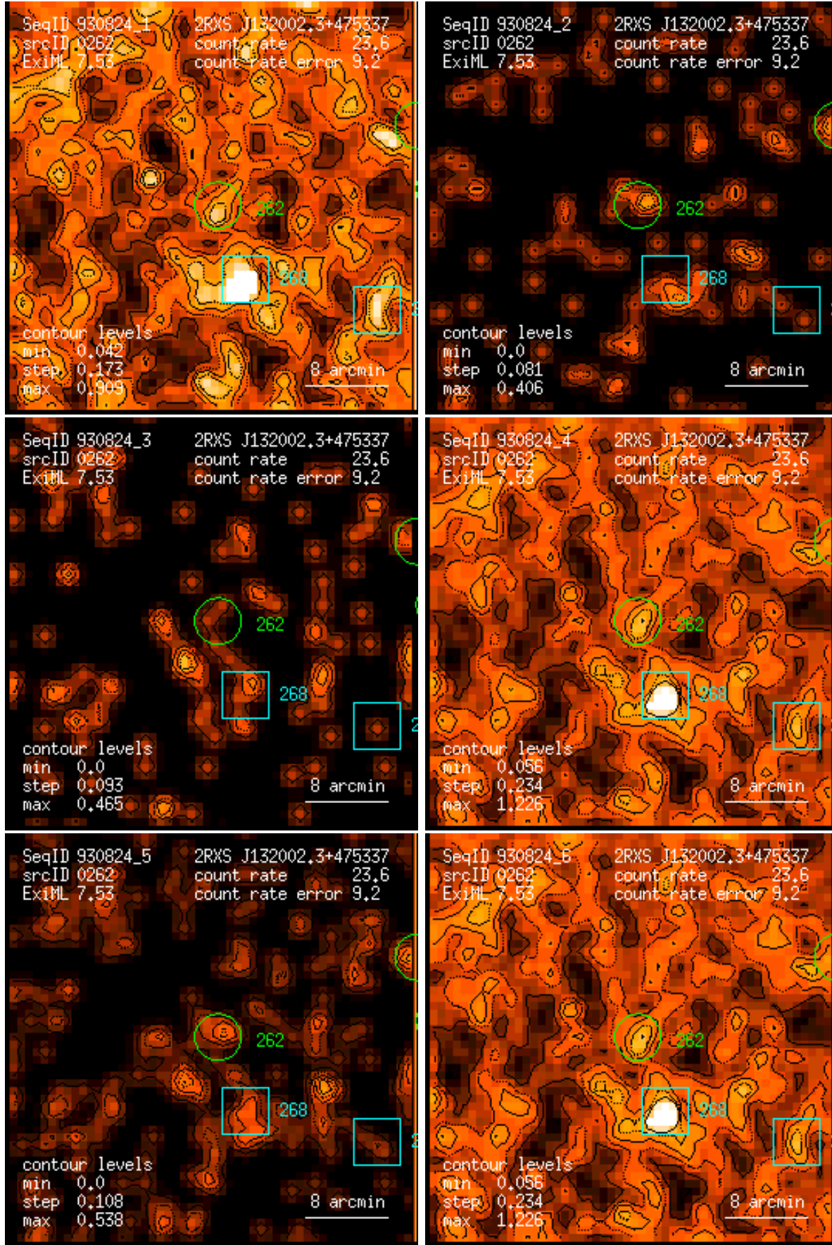
Figure 262: RASS 930824: detection 0262: band rate images, Gaussian filter: (1) PSPC channels 11 – 41, (2) 52 – 90, (3) 91 – 201, (4) 11 – 235, (5) 52 – 201, (6) 11 – 201. Broad band rates in counts/ks. Band rate contour levels in counts/ks/arcmin 2 .
