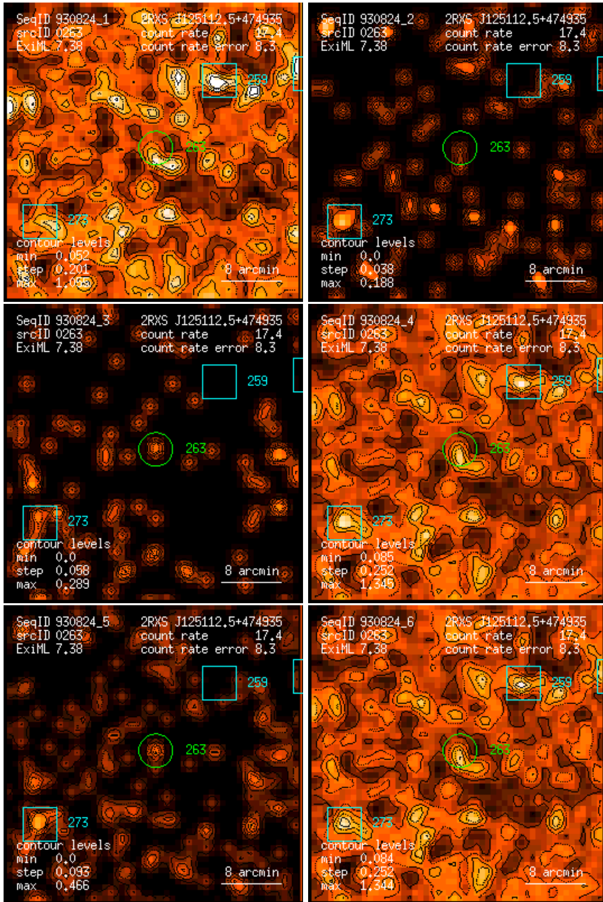
Figure 263: RASS 930824: detection 0263: band rate images, Gaussian filter: (1) PSPC channels 11 – 41, (2) 52 – 90, (3) 91 – 201, (4) 11 – 235, (5) 52 – 201, (6) 11 – 201. Broad band rates in counts/ks. Band rate contour levels in counts/ks/arcmin 2 .
