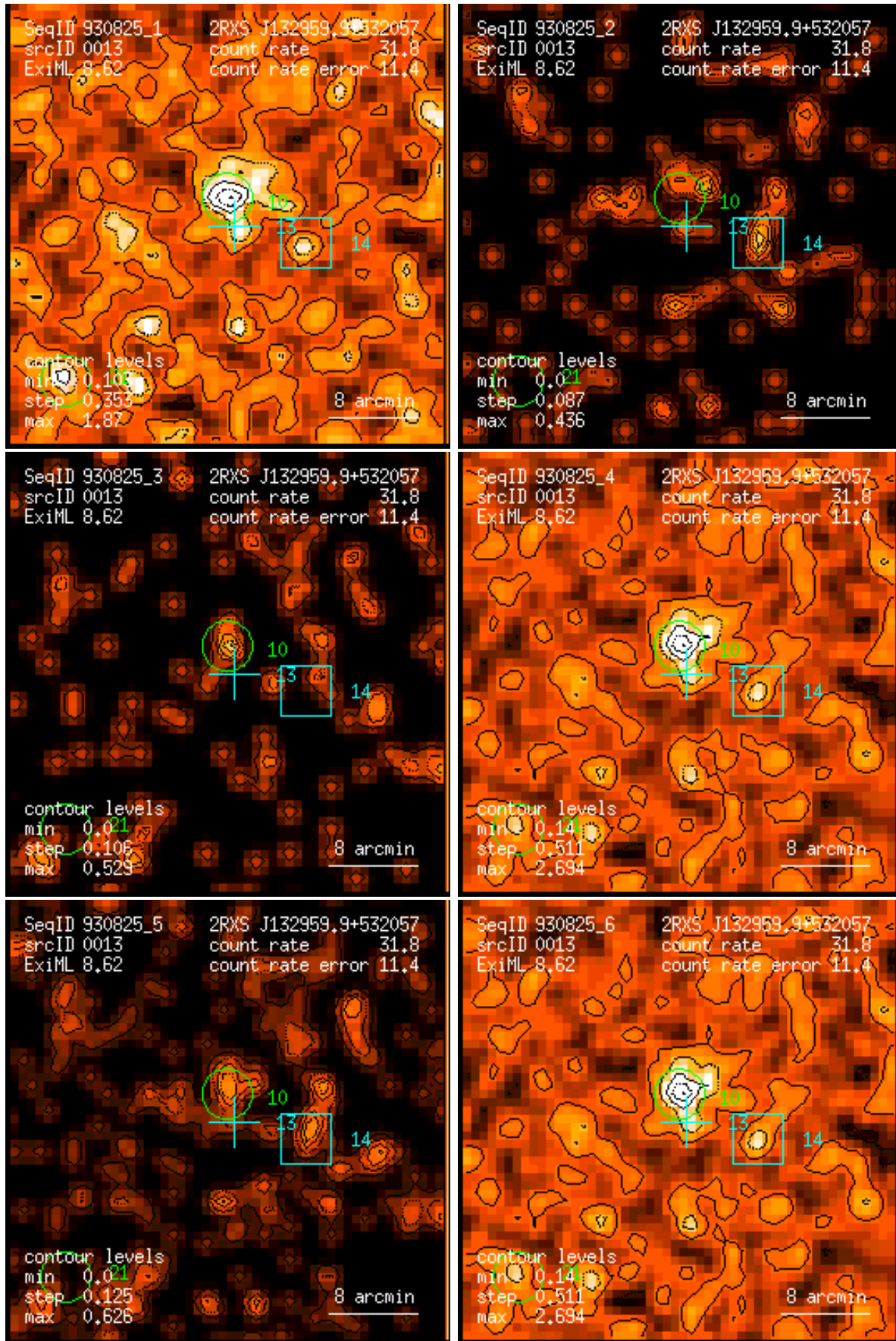
Figure 13: RASS 930825: detection 0013: band rate images, Gaussian filter: (1) PSPC channels 11 – 41, (2) 52 – 90, (3) 91 – 201, (4) 11 – 235, (5) 52 – 201, (6) 11 – 201. Broad band rates in counts/ks. Band rate contour levels in counts/ks/arcmin 2 .
