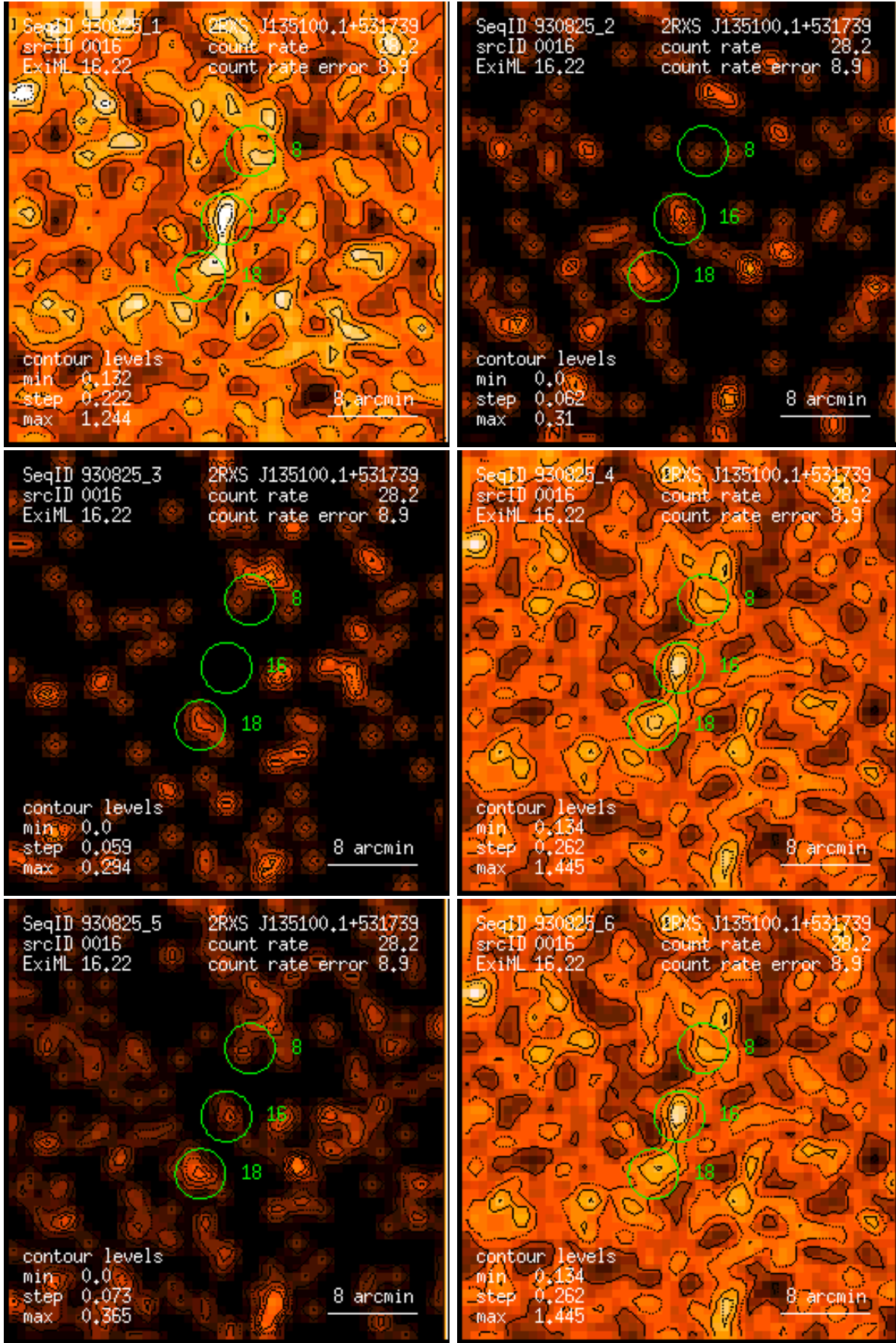
Figure 16: RASS 930825: detection 0016: band rate images, Gaussian filter: (1) PSPC channels 11 – 41, (2) 52 – 90, (3) 91 – 201, (4) 11 – 235, (5) 52 – 201, (6) 11 – 201. Broad band rates in counts/ks. Band rate contour levels in counts/ks/arcmin 2 .
