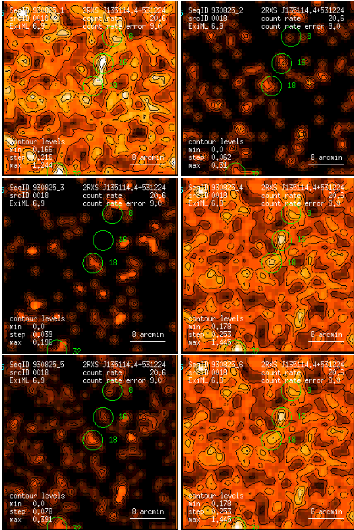
Figure 18: RASS 930825: detection 0018: band rate images, Gaussian filter: (1) PSPC channels 11 – 41, (2) 52 – 90, (3) 91 – 201, (4) 11 – 235, (5) 52 – 201, (6) 11 – 201. Broad band rates in counts/ks. Band rate contour levels in counts/ks/arcmin 2 .
