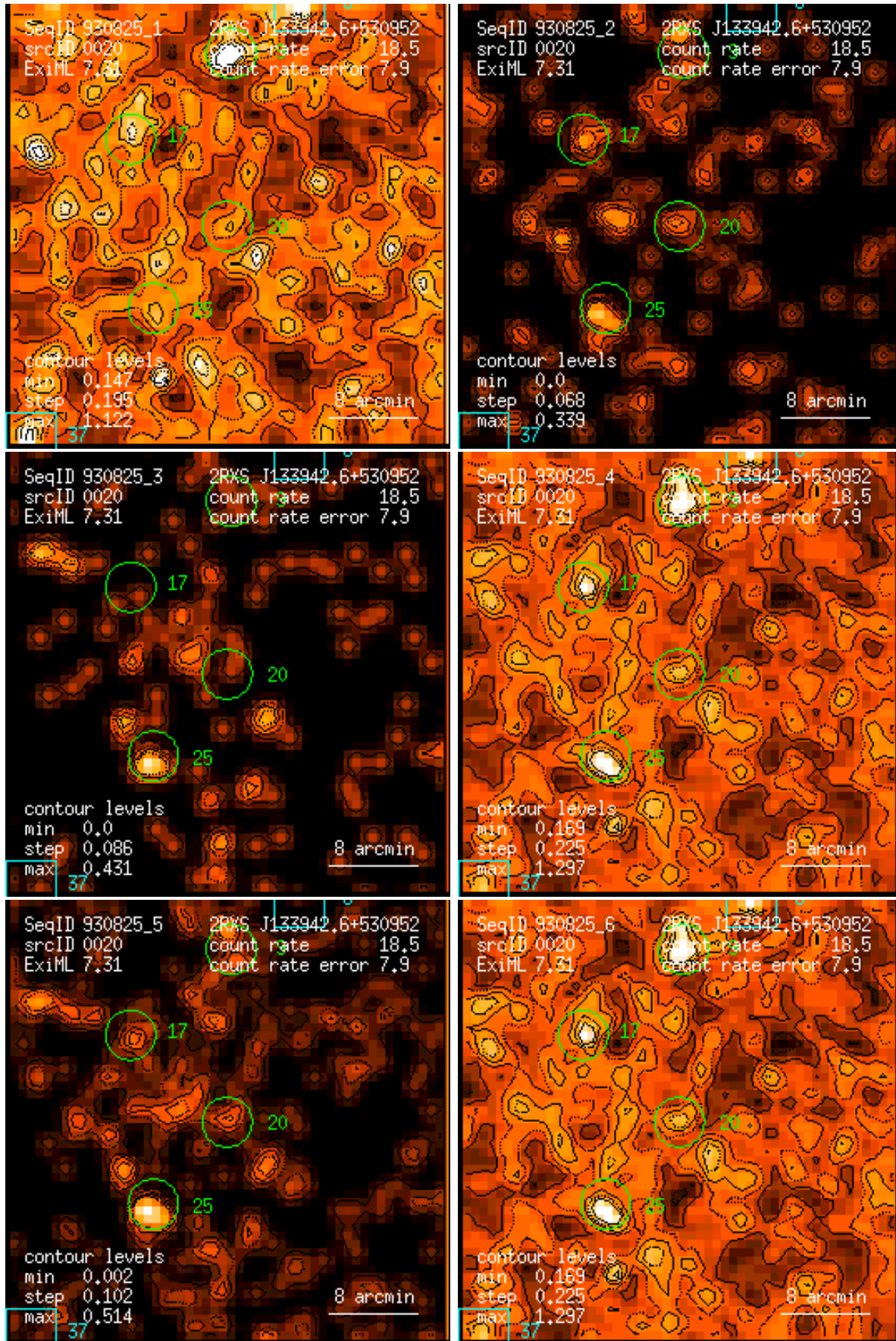
Figure 20: RASS 930825: detection 0020: band rate images, Gaussian filter: (1) PSPC channels 11 – 41, (2) 52 – 90, (3) 91 – 201, (4) 11 – 235, (5) 52 – 201, (6) 11 – 201. Broad band rates in counts/ks. Band rate contour levels in counts/ks/arcmin 2 .
