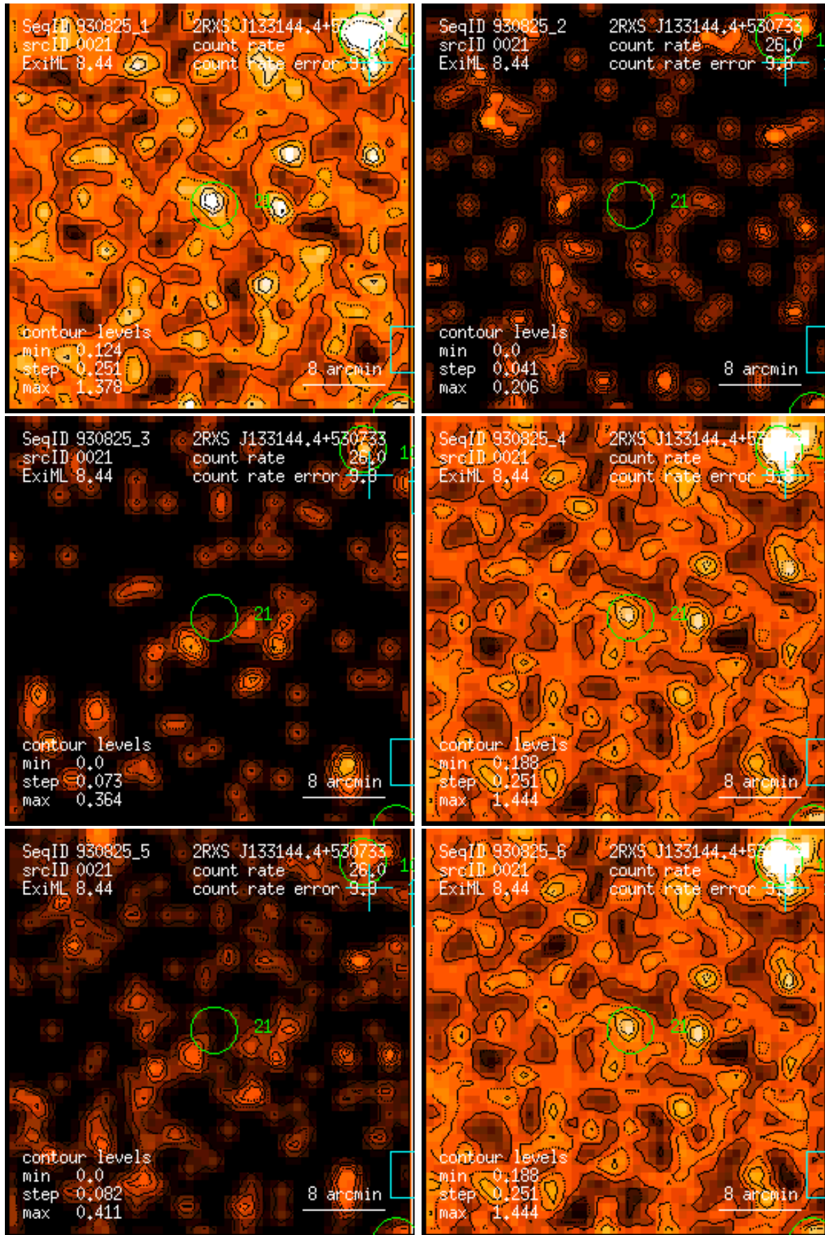
Figure 21: RASS 930825: detection 0021: band rate images, Gaussian filter: (1) PSPC channels 11 – 41, (2) 52 – 90, (3) 91 – 201, (4) 11 – 235, (5) 52 – 201, (6) 11 – 201. Broad band rates in counts/ks. Band rate contour levels in counts/ks/arcmin 2 .
