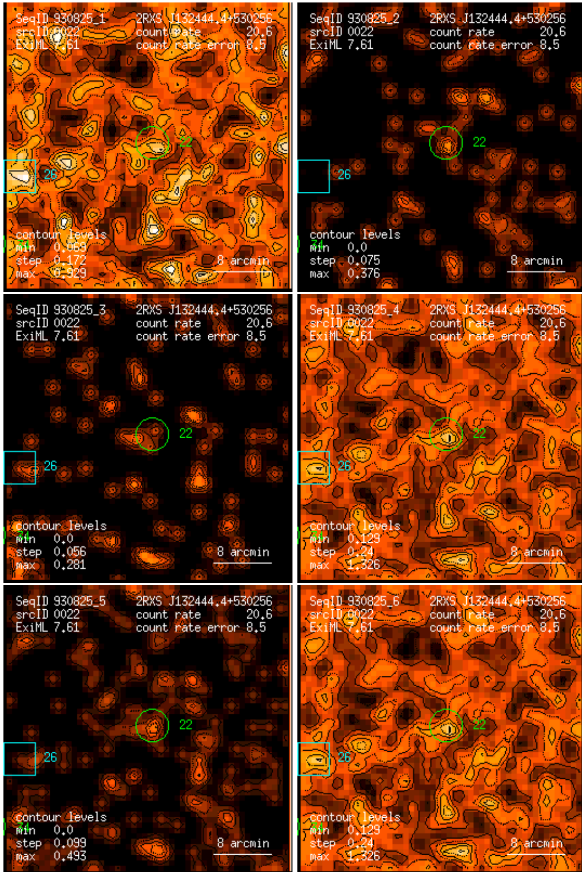
Figure 22: RASS 930825: detection 0022: band rate images, Gaussian filter: (1) PSPC channels 11 – 41, (2) 52 – 90, (3) 91 – 201, (4) 11 – 235, (5) 52 – 201, (6) 11 – 201. Broad band rates in counts/ks. Band rate contour levels in counts/ks/arcmin 2 .
