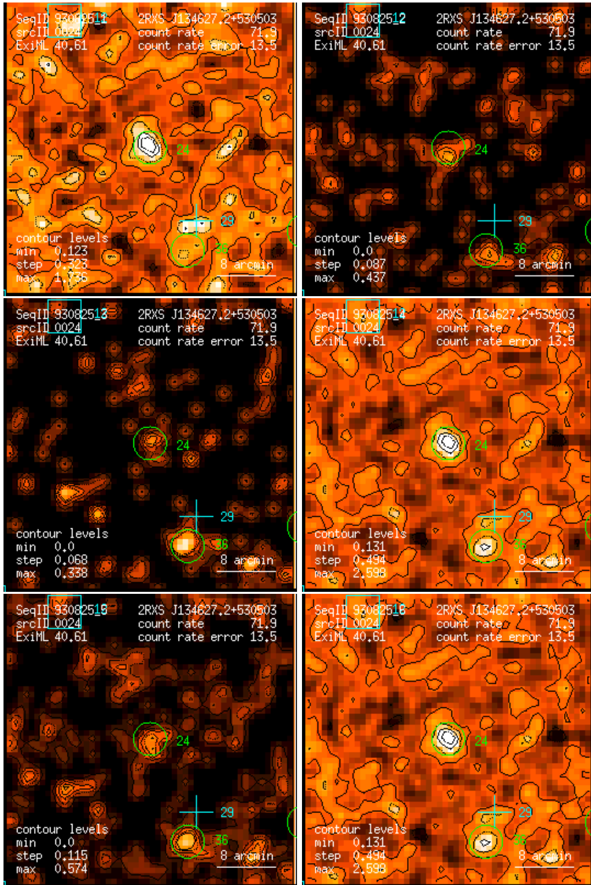
Figure 24: RASS 930825: detection 0024: band rate images, Gaussian filter: (1) PSPC channels 11 – 41, (2) 52 – 90, (3) 91 – 201, (4) 11 – 235, (5) 52 – 201, (6) 11 – 201. Broad band rates in counts/ks. Band rate contour levels in counts/ks/arcmin 2 .
