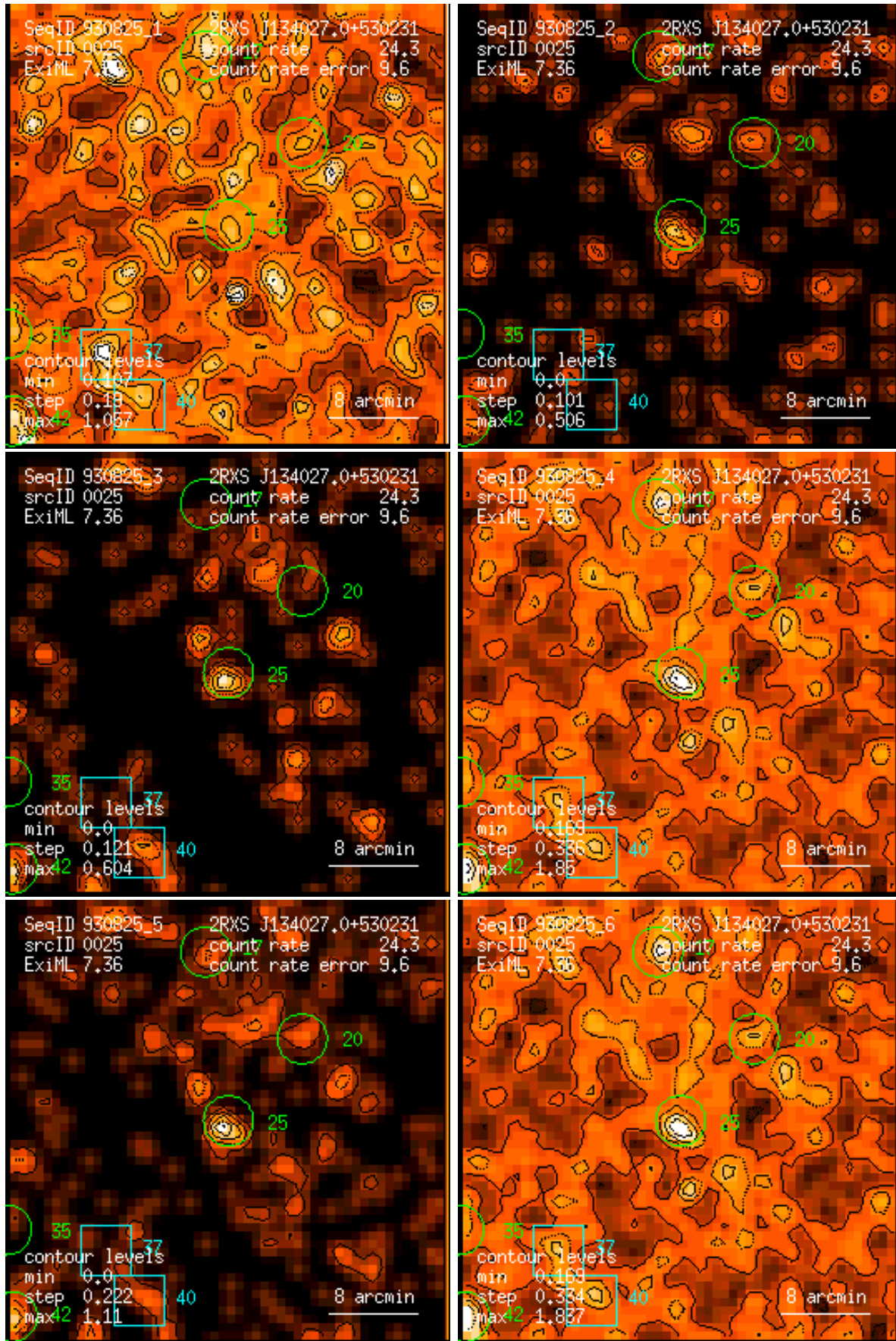
Figure 25: RASS 930825: detection 0025: band rate images, Gaussian filter: (1) PSPC channels 11 – 41, (2) 52 – 90, (3) 91 – 201, (4) 11 – 235, (5) 52 – 201, (6) 11 – 201. Broad band rates in counts/ks. Band rate contour levels in counts/ks/arcmin 2 .
