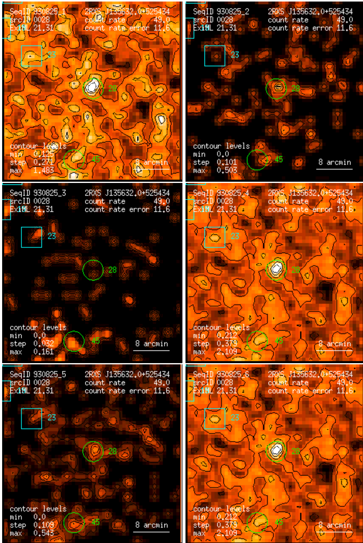
Figure 28: RASS 930825: detection 0028: band rate images, Gaussian filter: (1) PSPC channels 11 – 41, (2) 52 – 90, (3) 91 – 201, (4) 11 – 235, (5) 52 – 201, (6) 11 – 201. Broad band rates in counts/ks. Band rate contour levels in counts/ks/arcmin 2 .
