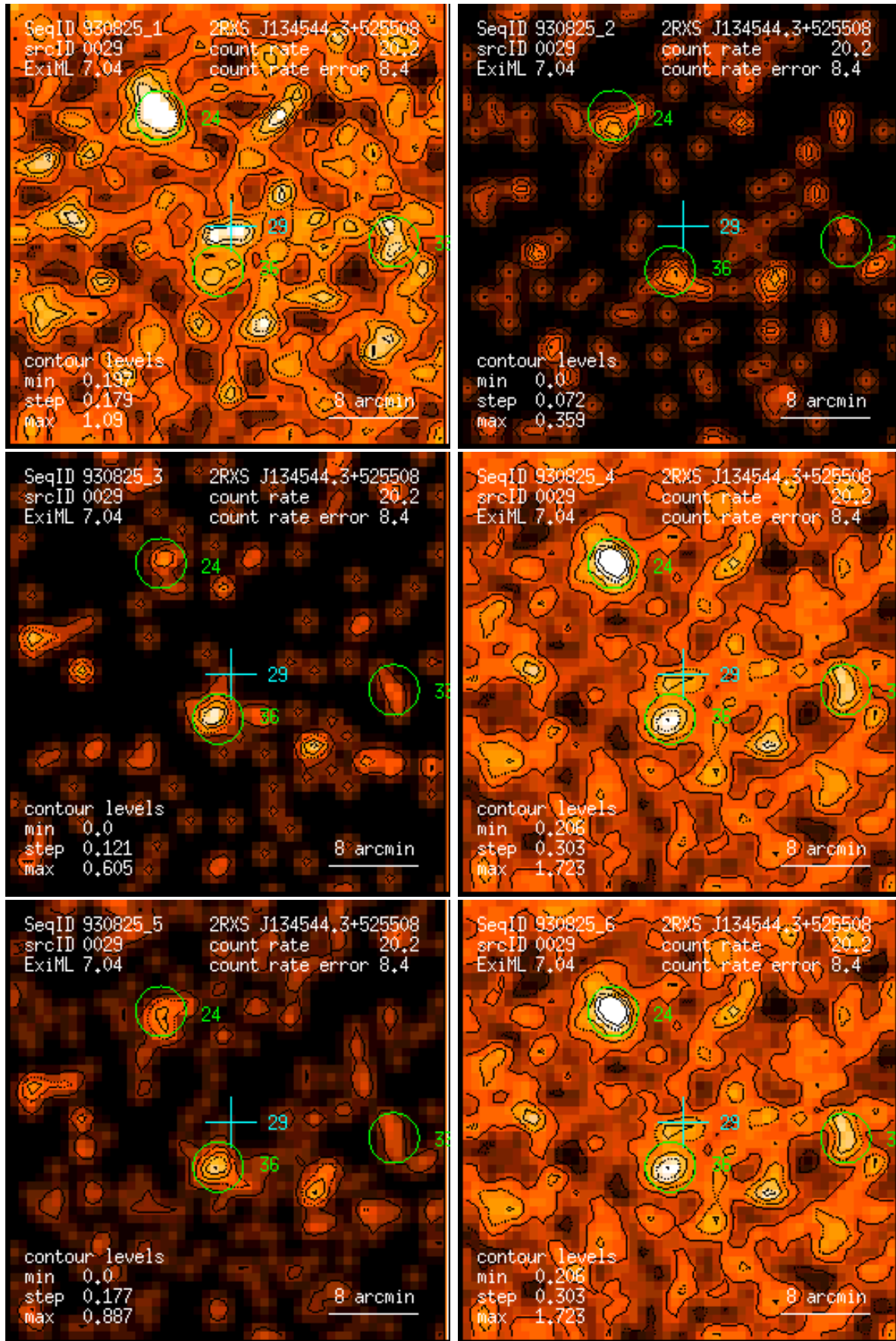
Figure 29: RASS 930825: detection 0029: band rate images, Gaussian filter: (1) PSPC channels 11 – 41, (2) 52 – 90, (3) 91 – 201, (4) 11 – 235, (5) 52 – 201, (6) 11 – 201. Broad band rates in counts/ks. Band rate contour levels in counts/ks/arcmin 2 .
