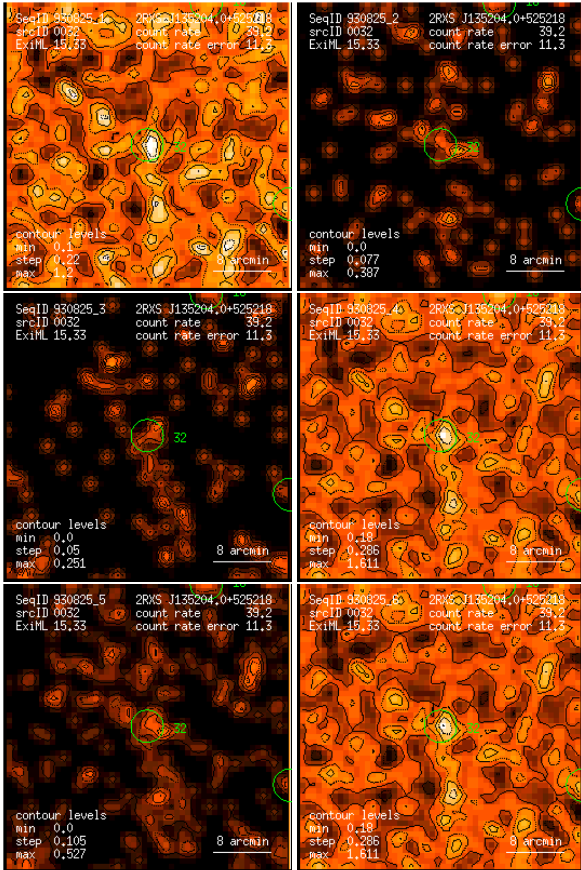
Figure 32: RASS 930825: detection 0032: band rate images, Gaussian filter: (1) PSPC channels 11 – 41, (2) 52 – 90, (3) 91 – 201, (4) 11 – 235, (5) 52 – 201, (6) 11 – 201. Broad band rates in counts/ks. Band rate contour levels in counts/ks/arcmin 2 .
