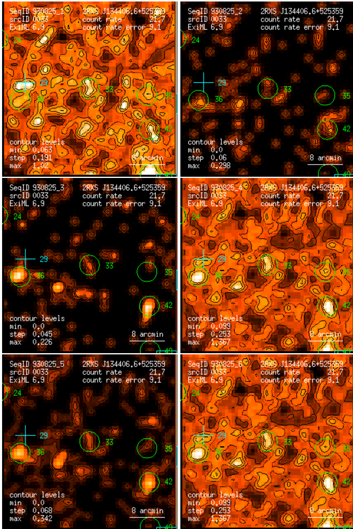
Figure 33: RASS 930825: detection 0033: band rate images, Gaussian filter: (1) PSPC channels 11 – 41, (2) 52 – 90, (3) 91 – 201, (4) 11 – 235, (5) 52 – 201, (6) 11 – 201. Broad band rates in counts/ks. Band rate contour levels in counts/ks/arcmin 2 .
