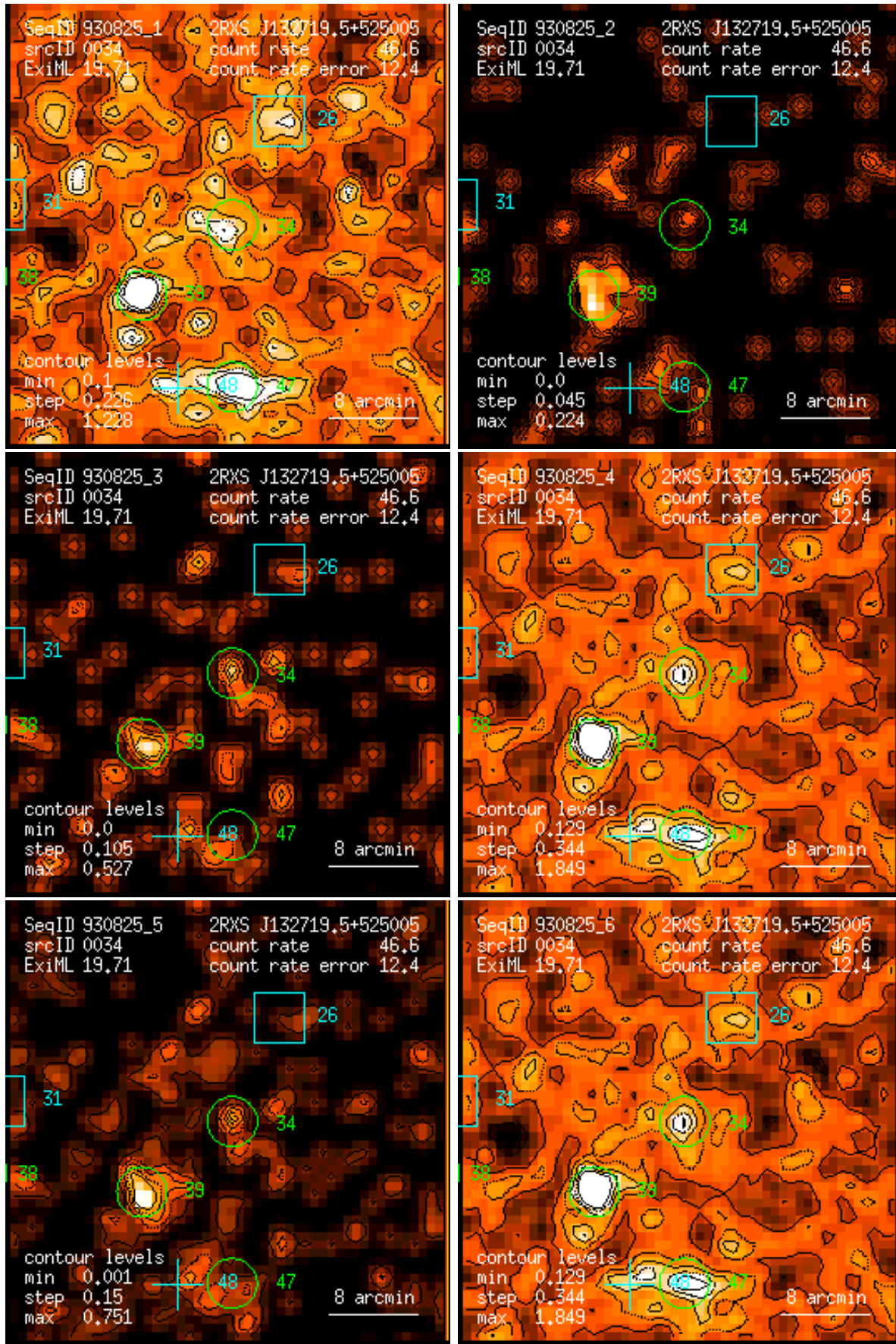
Figure 34: RASS 930825: detection 0034: band rate images, Gaussian filter: (1) PSPC channels 11 – 41, (2) 52 – 90, (3) 91 – 201, (4) 11 – 235, (5) 52 – 201, (6) 11 – 201. Broad band rates in counts/ks. Band rate contour levels in counts/ks/arcmin 2 .
