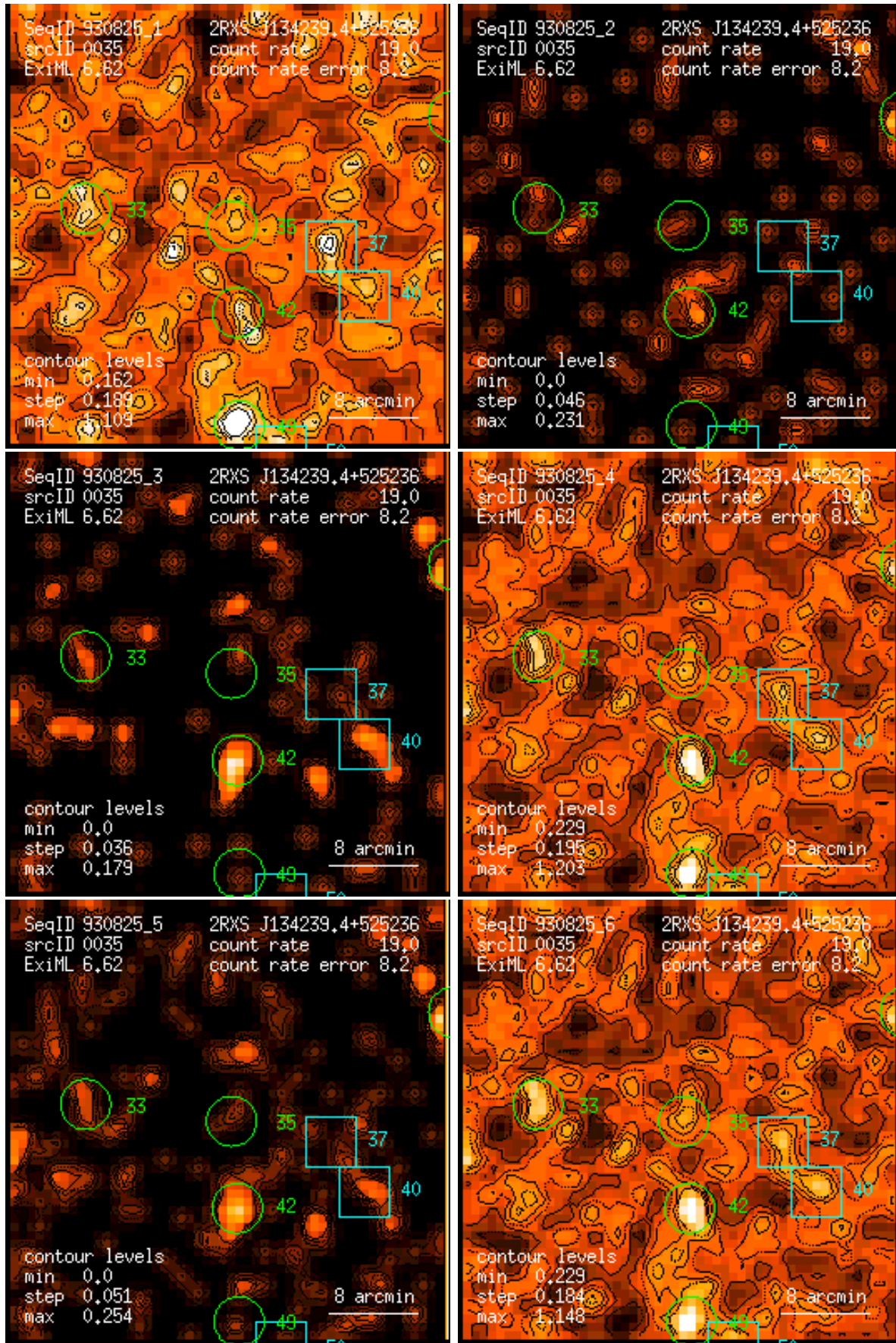
Figure 35: RASS 930825: detection 0035: band rate images, Gaussian filter: (1) PSPC channels 11 – 41, (2) 52 – 90, (3) 91 – 201, (4) 11 – 235, (5) 52 – 201, (6) 11 – 201. Broad band rates in counts/ks. Band rate contour levels in counts/ks/arcmin 2 .
