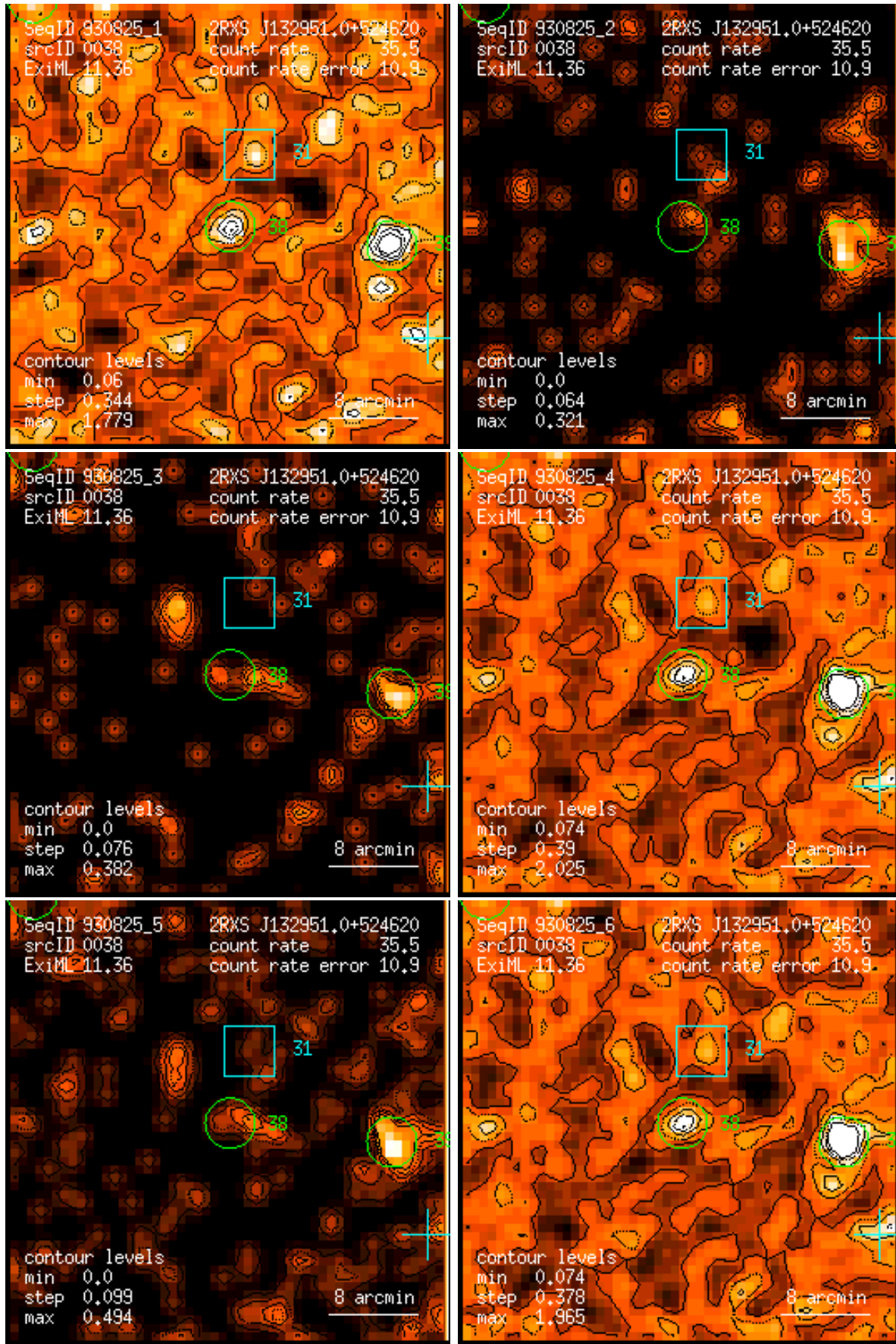
Figure 38: RASS 930825: detection 0038: band rate images, Gaussian filter: (1) PSPC channels 11 – 41, (2) 52 – 90, (3) 91 – 201, (4) 11 – 235, (5) 52 – 201, (6) 11 – 201. Broad band rates in counts/ks. Band rate contour levels in counts/ks/arcmin 2 .
