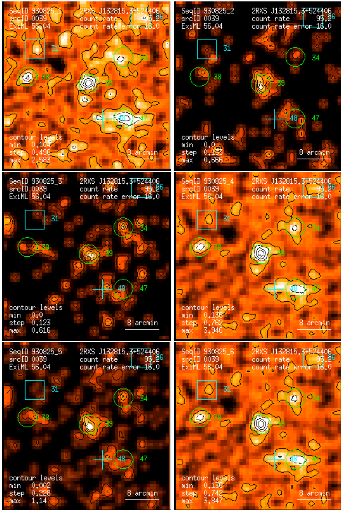
Figure 39: RASS 930825: detection 0039: band rate images, Gaussian filter: (1) PSPC channels 11 – 41, (2) 52 – 90, (3) 91 – 201, (4) 11 – 235, (5) 52 – 201, (6) 11 – 201. Broad band rates in counts/ks. Band rate contour levels in counts/ks/arcmin 2 .
