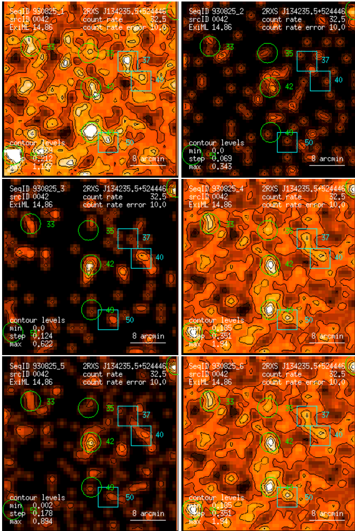
Figure 42: RASS 930825: detection 0042: band rate images, Gaussian filter: (1) PSPC channels 11 – 41, (2) 52 – 90, (3) 91 – 201, (4) 11 – 235, (5) 52 – 201, (6) 11 – 201. Broad band rates in counts/ks. Band rate contour levels in counts/ks/arcmin 2 .
