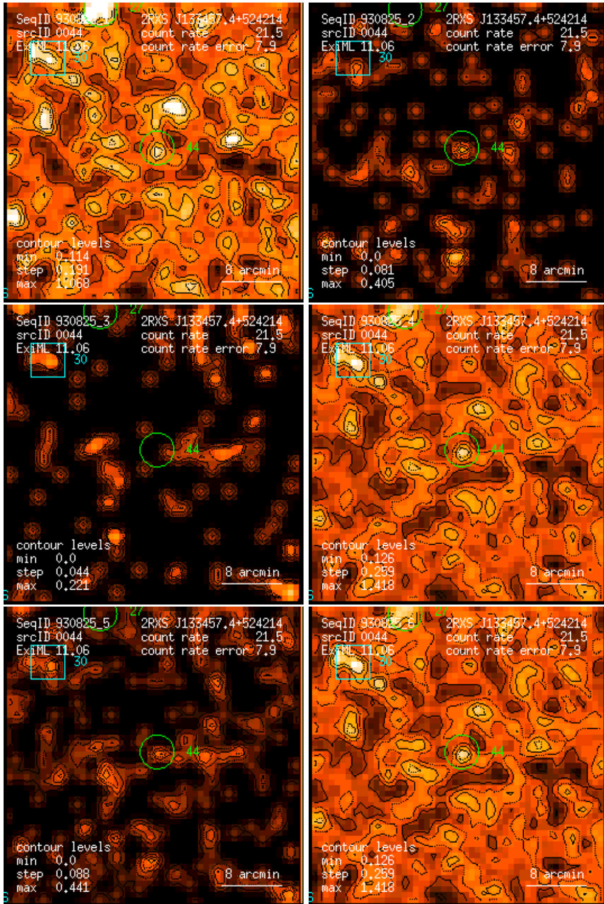
Figure 44: RASS 930825: detection 0044: band rate images, Gaussian filter: (1) PSPC channels 11 – 41, (2) 52 – 90, (3) 91 – 201, (4) 11 – 235, (5) 52 – 201, (6) 11 – 201. Broad band rates in counts/ks. Band rate contour levels in counts/ks/arcmin 2 .
