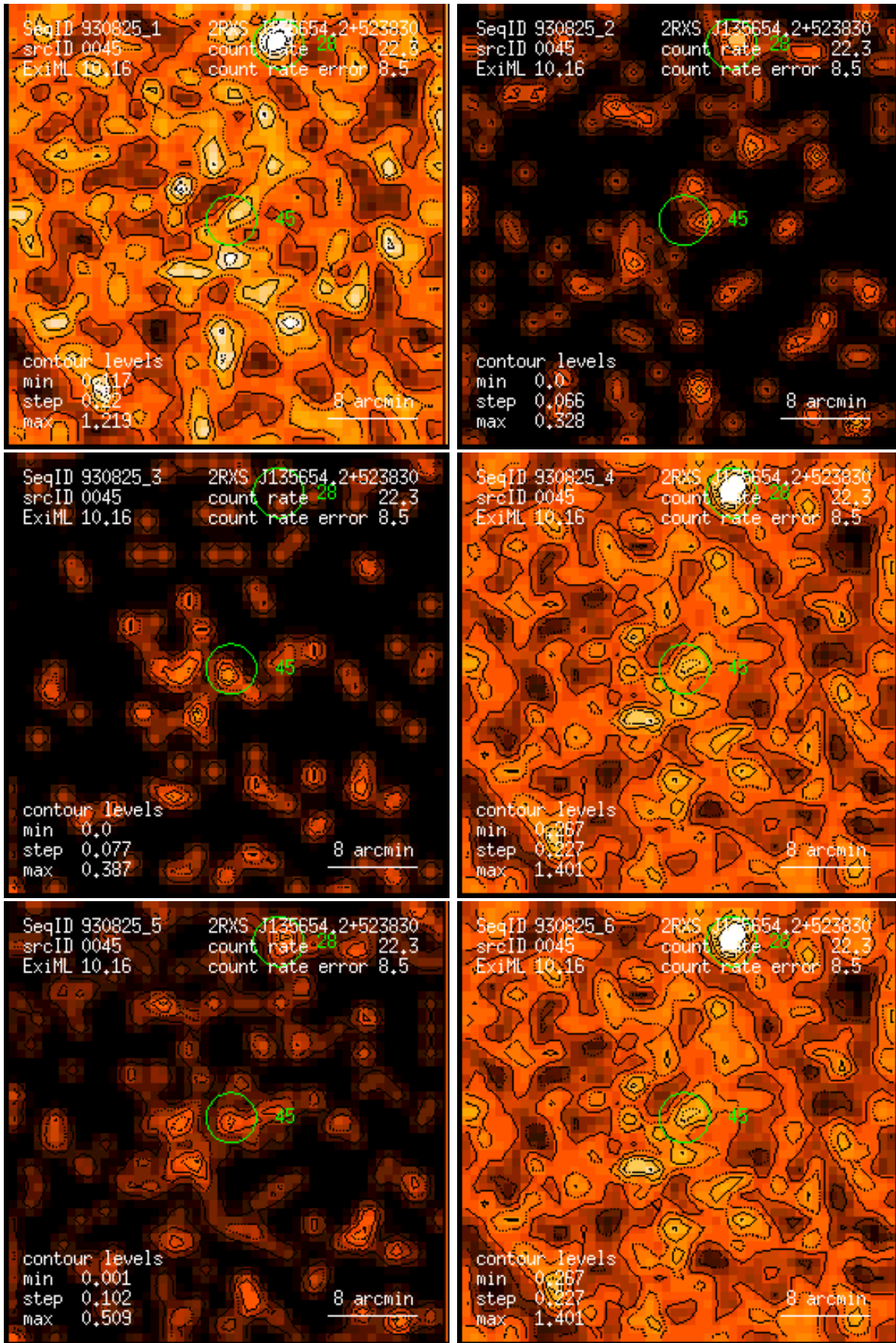
Figure 45: RASS 930825: detection 0045: band rate images, Gaussian filter: (1) PSPC channels 11 – 41, (2) 52 – 90, (3) 91 – 201, (4) 11 – 235, (5) 52 – 201, (6) 11 – 201. Broad band rates in counts/ks. Band rate contour levels in counts/ks/arcmin 2 .
