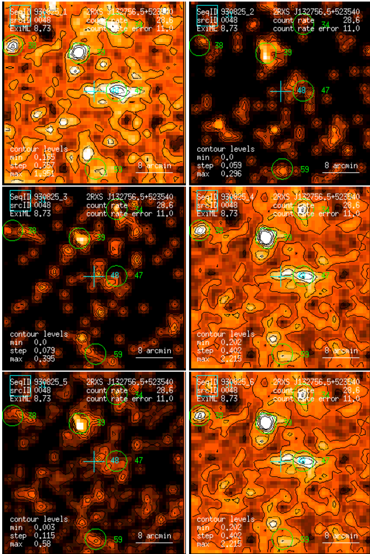
Figure 48: RASS 930825: detection 0048: band rate images, Gaussian filter: (1) PSPC channels 11 – 41, (2) 52 – 90, (3) 91 – 201, (4) 11 – 235, (5) 52 – 201, (6) 11 – 201. Broad band rates in counts/ks. Band rate contour levels in counts/ks/arcmin 2 .
