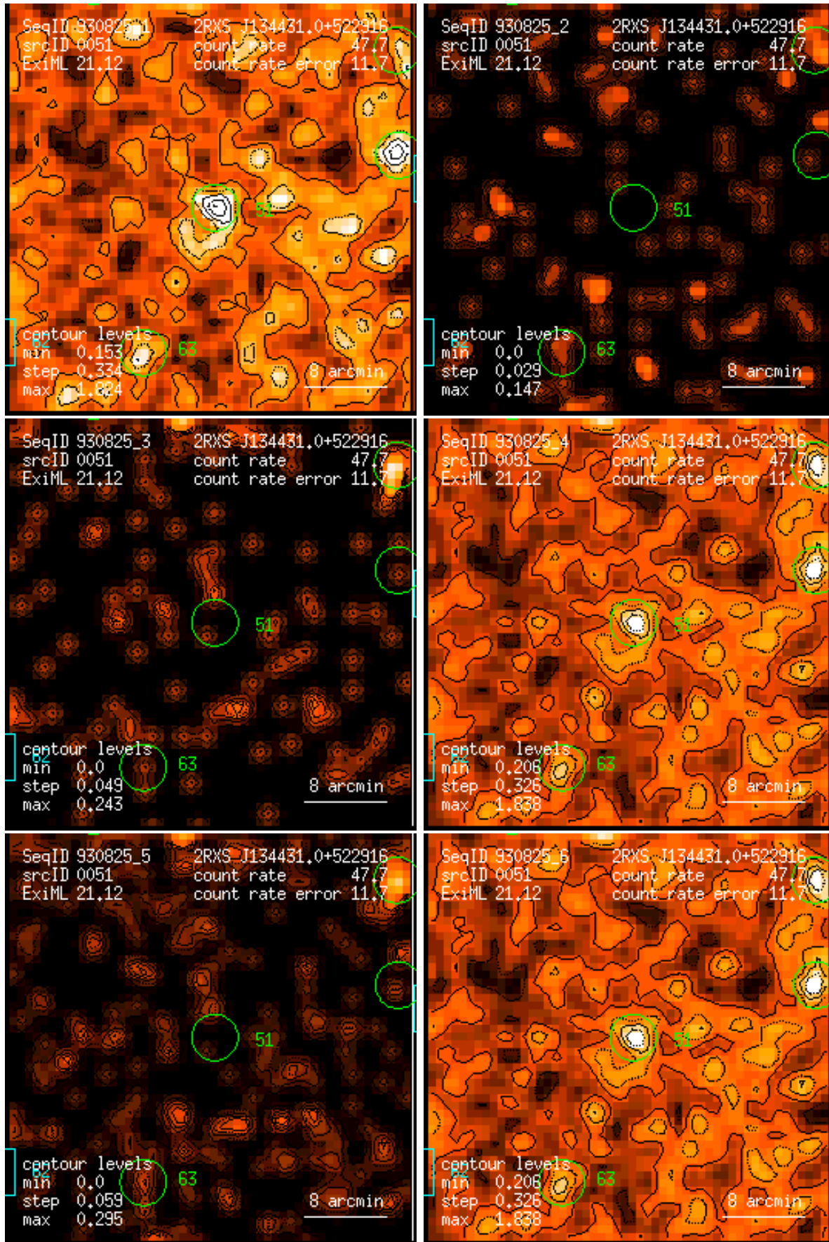
Figure 51: RASS 930825: detection 0051: band rate images, Gaussian filter: (1) PSPC channels 11 – 41, (2) 52 – 90, (3) 91 – 201, (4) 11 – 235, (5) 52 – 201, (6) 11 – 201. Broad band rates in counts/ks. Band rate contour levels in counts/ks/arcmin 2 .
