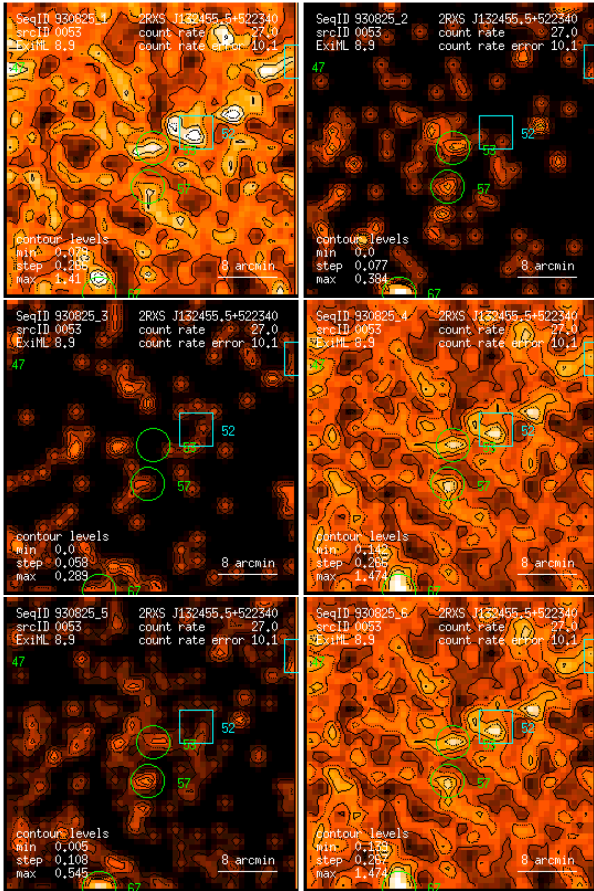
Figure 53: RASS 930825: detection 0053: band rate images, Gaussian filter: (1) PSPC channels 11 – 41, (2) 52 – 90, (3) 91 – 201, (4) 11 – 235, (5) 52 – 201, (6) 11 – 201. Broad band rates in counts/ks. Band rate contour levels in counts/ks/arcmin 2 .
