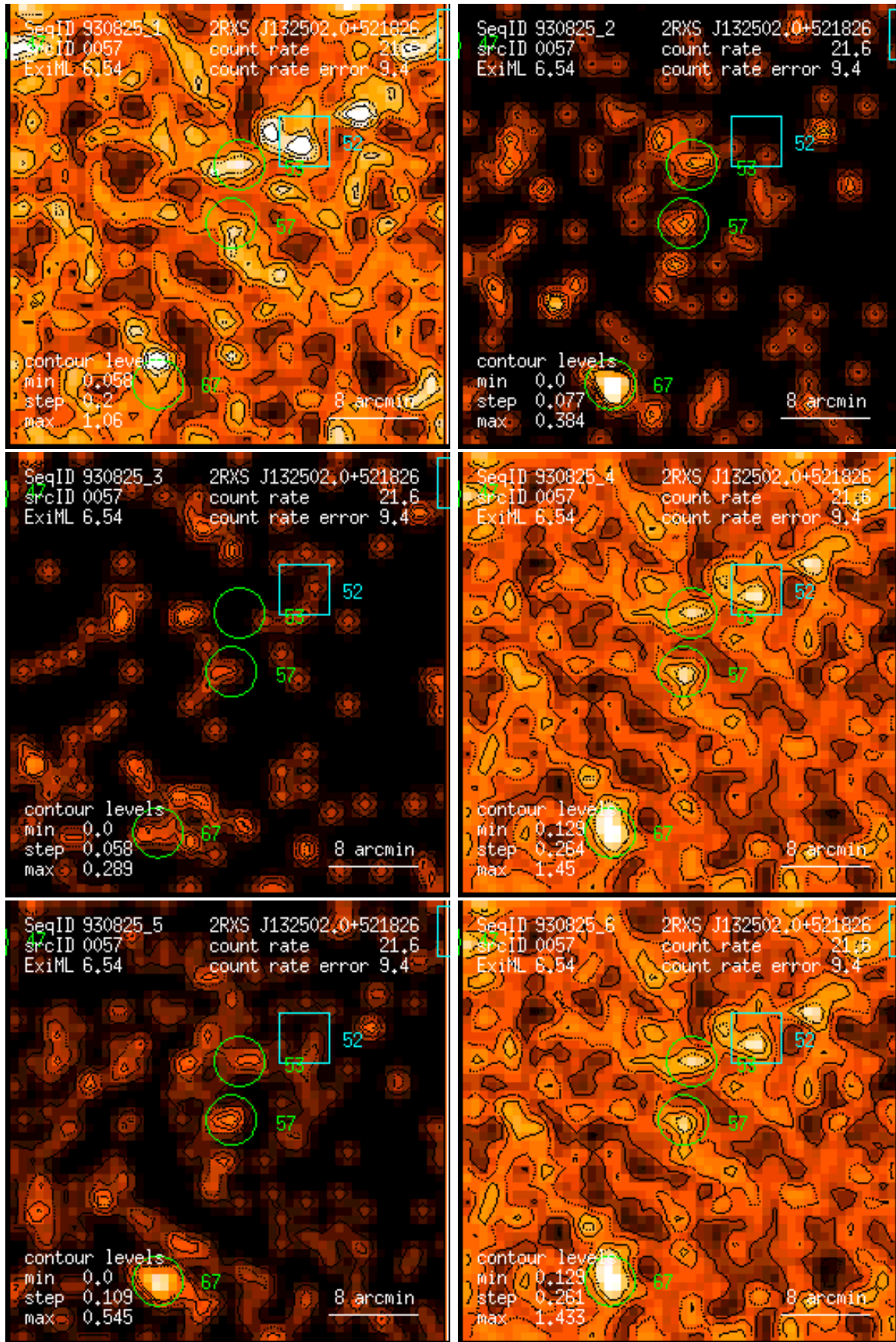
Figure 57: RASS 930825: detection 0057: band rate images, Gaussian filter: (1) PSPC channels 11 – 41, (2) 52 – 90, (3) 91 – 201, (4) 11 – 235, (5) 52 – 201, (6) 11 – 201. Broad band rates in counts/ks. Band rate contour levels in counts/ks/arcmin 2 .
