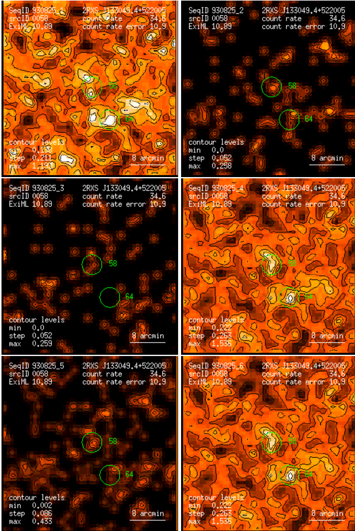
Figure 58: RASS 930825: detection 0058: band rate images, Gaussian filter: (1) PSPC channels 11 – 41, (2) 52 – 90, (3) 91 – 201, (4) 11 – 235, (5) 52 – 201, (6) 11 – 201. Broad band rates in counts/ks. Band rate contour levels in counts/ks/arcmin 2 .
